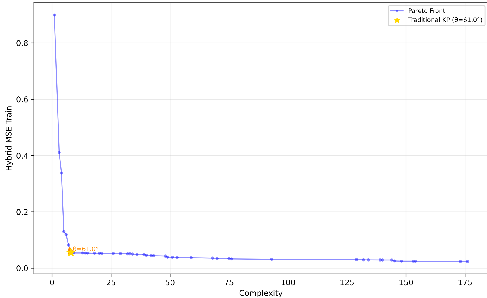
519_vinnie - Run 4 - MVP - Hybrid MSE Train \lambda_1=0.00, \lambda_2=0.10, \lambda_3=0.00 | Difficulty: 1.00 | Method: hmr
