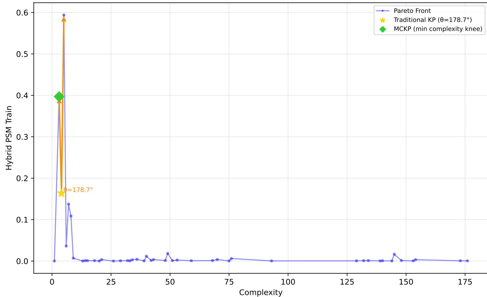
519_vinnie - Run 4 - MVP - Hybrid PSM Train \lambda_1=0.00, \lambda_2=0.10, \lambda_3=0.00 | Difficulty: 1.00 | Method: hmr
