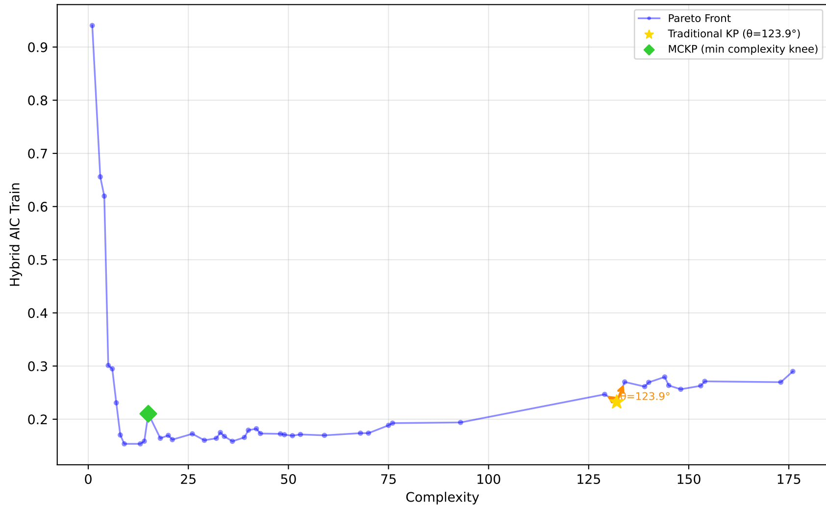
519_vinnie - Run 4 - SVP - Hybrid AIC Train \lambda_1=1.00, \lambda_2=1.00, \lambda_3=1.00 | Difficulty: 1.00 | Method: hmr
