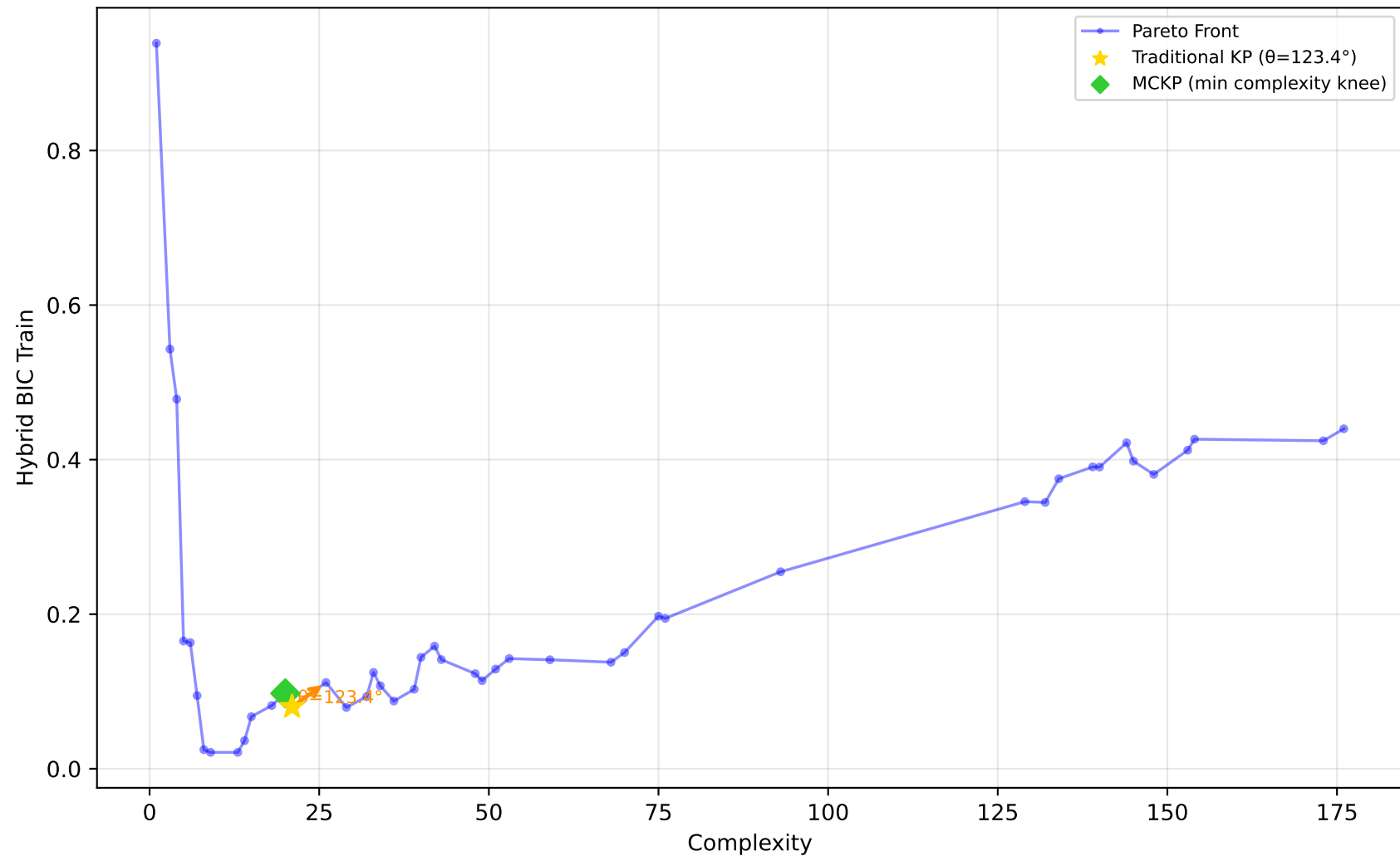
519_vinnie - Run 4 - SVP - Hybrid BIC Train \lambda_1=0.00, \lambda_2=0.00, \lambda_3=0.00 | Difficulty: 1.00 | Method: hmr
