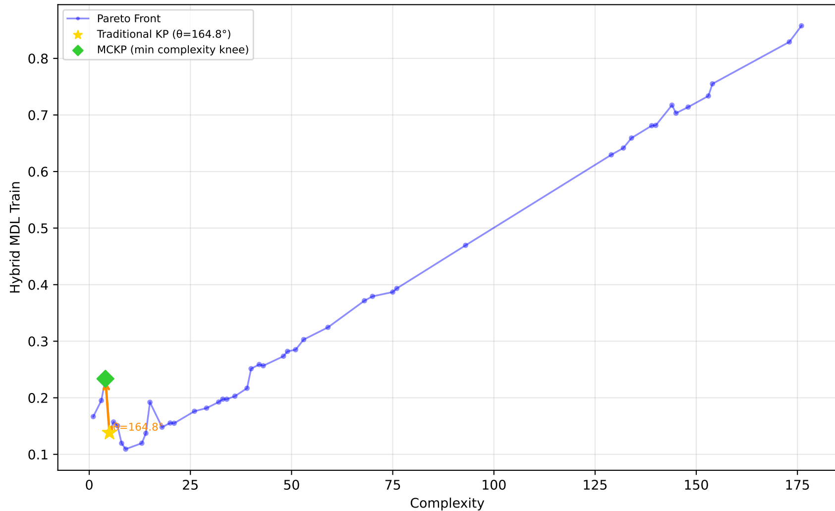
519_vinnie - Run 4 - SVP - Hybrid MDL Train \lambda_1=1.00, \lambda_2=1.00, \lambda_3=1.00 | Difficulty: 1.00 | Method: hmr
