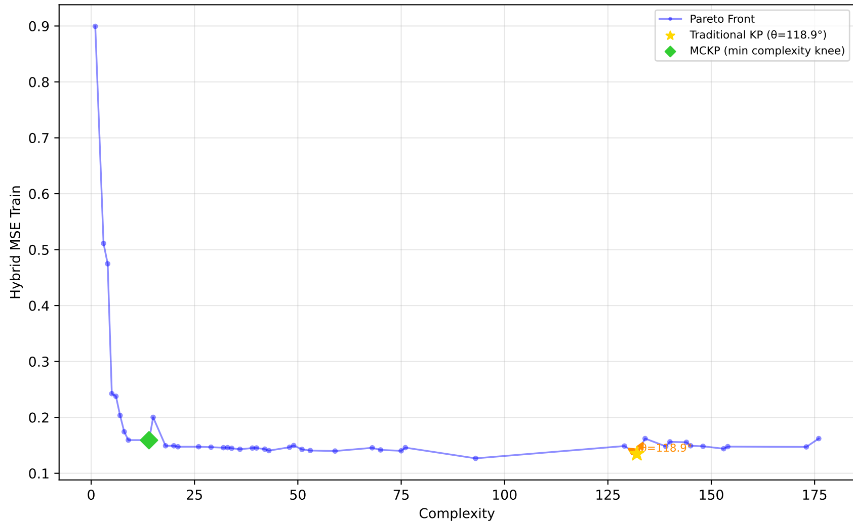
519_vinnie - Run 4 - SVP - Hybrid MSE Train \lambda_1=1.00, \lambda_2=1.00, \lambda_3=1.00 | Difficulty: 1.00 | Method: hmr
