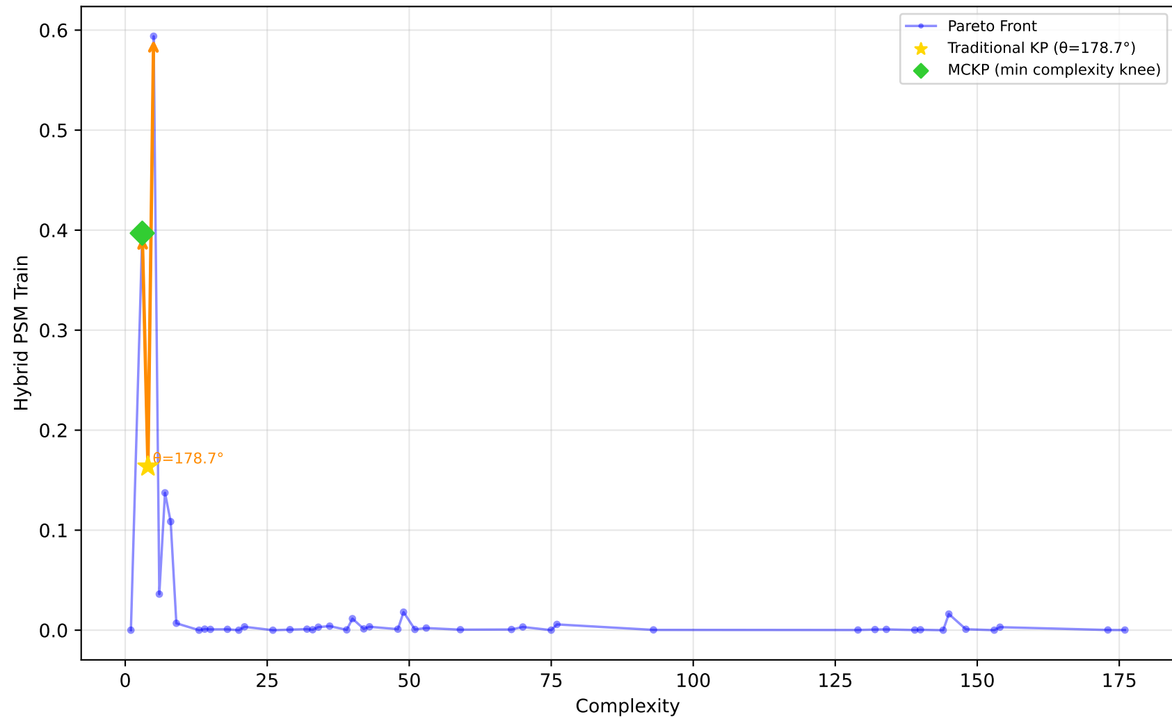
519_vinnie - Run 4 - SVP - Hybrid PSM Train \lambda_1=0.00, \lambda_2=0.00, \lambda_3=0.00 | Difficulty: 1.00 | Method: hmr
