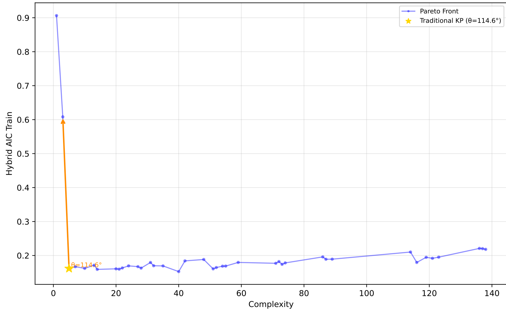
519_vinnie - Run 5 - MVP - Hybrid AIC Train \lambda_1=1.00, \lambda_2=0.00, \lambda_3=1.00 | Difficulty: 0.50 | Method: mckp
