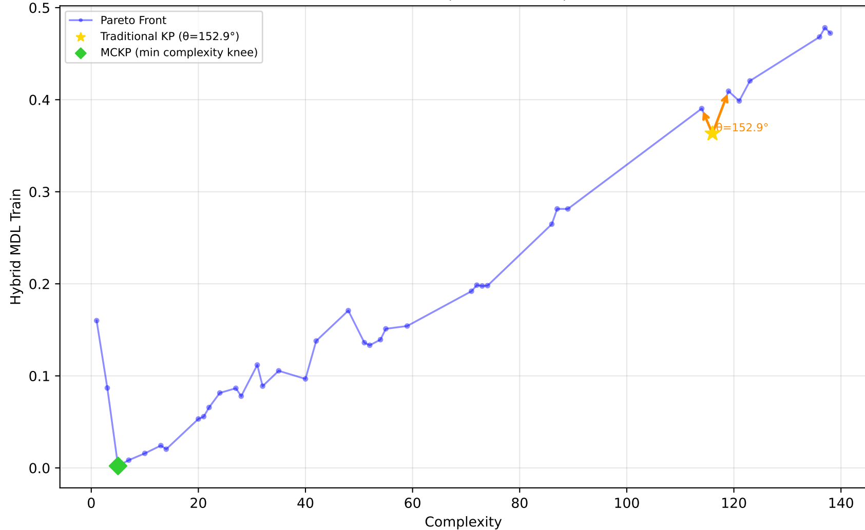
519_vinnie - Run 5 - MVP - Hybrid MDL Train \lambda_1=0.00, \lambda_2=0.10, \lambda_3=0.00 | Difficulty: 0.50 | Method: mckp
