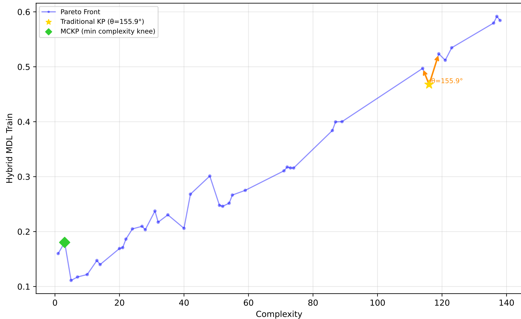
519_vinnie - Run 5 - MVP - Hybrid MDL Train \lambda_1=1.00, \lambda_2=0.00, \lambda_3=1.00 | Difficulty: 0.50 | Method: mckp
