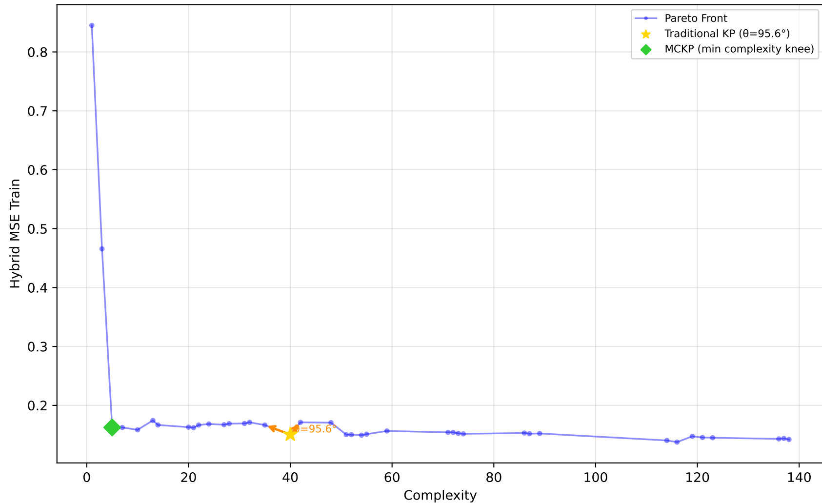
519_vinnie - Run 5 - MVP - Hybrid MSE Train \lambda_1=1.00, \lambda_2=0.00, \lambda_3=1.00 | Difficulty: 0.50 | Method: mckp
