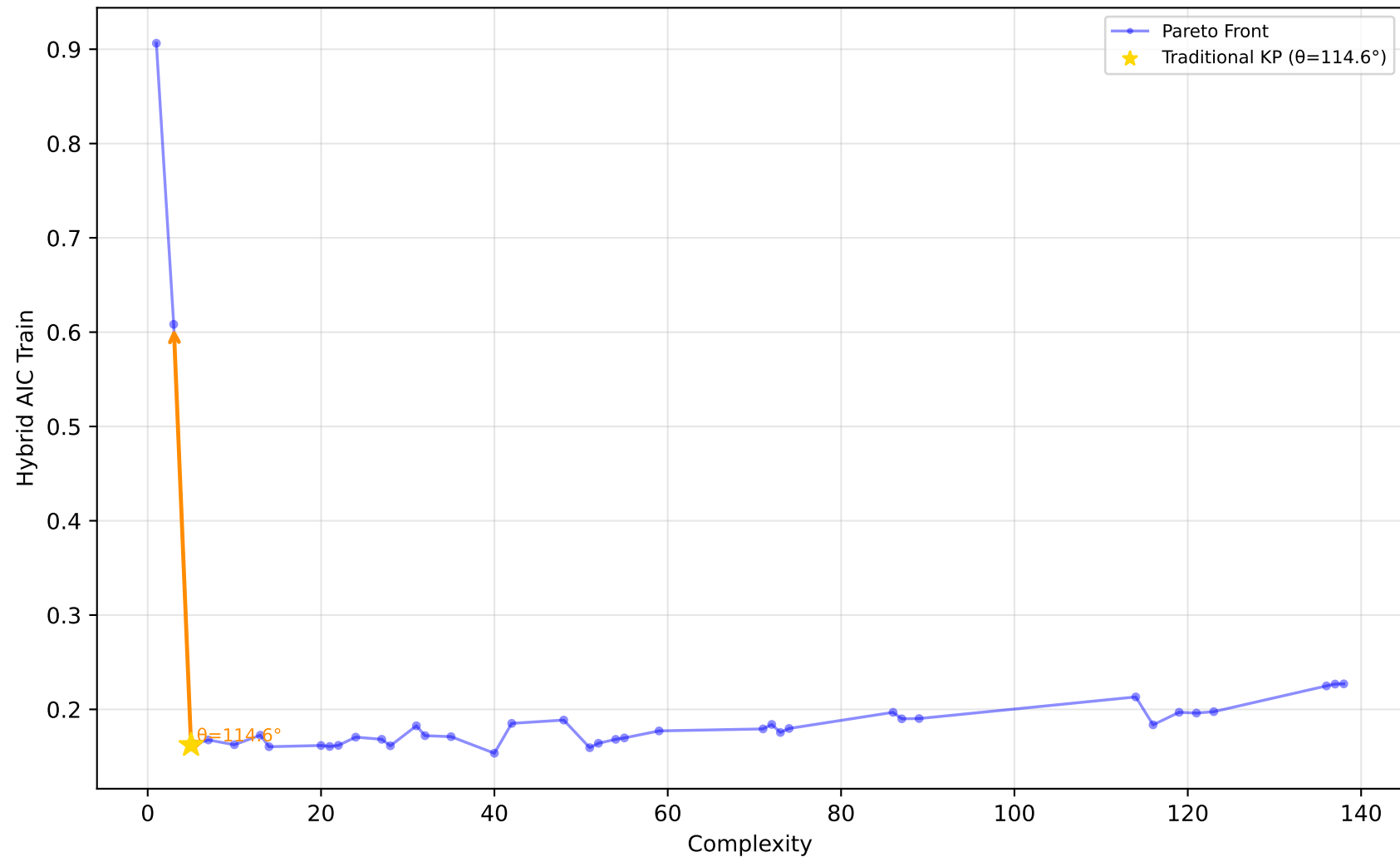
519_vinnie - Run 5 - SVP - Hybrid AIC Train \lambda_1=1.00 , \lambda_2=1.00 , \lambda_3=1.00 | Difficulty: 0.50 | Method: mckp
