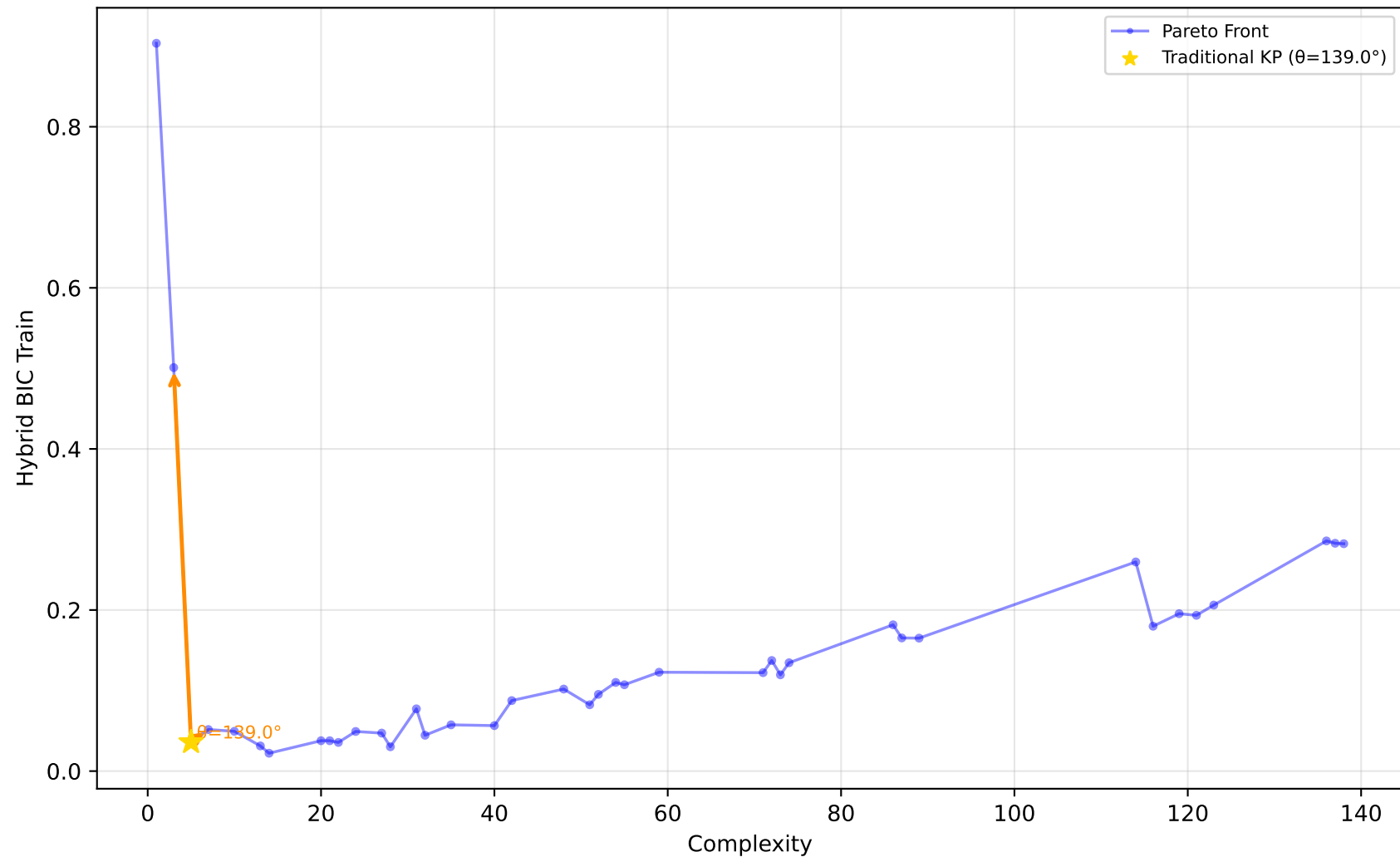
519_vinnie - Run 5 - SVP - Hybrid BIC Train \lambda_1=0.00, \lambda_2=0.00, \lambda_3=0.00 | Difficulty: 0.50 | Method: mckp
