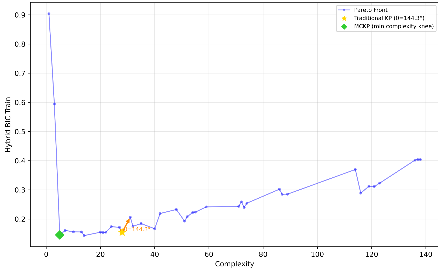
519_vinnie - Run 5 - SVP - Hybrid BIC Train \lambda_1=1.00, \lambda_2=1.00, \lambda_3=1.00 | Difficulty: 0.50 | Method: mckp
