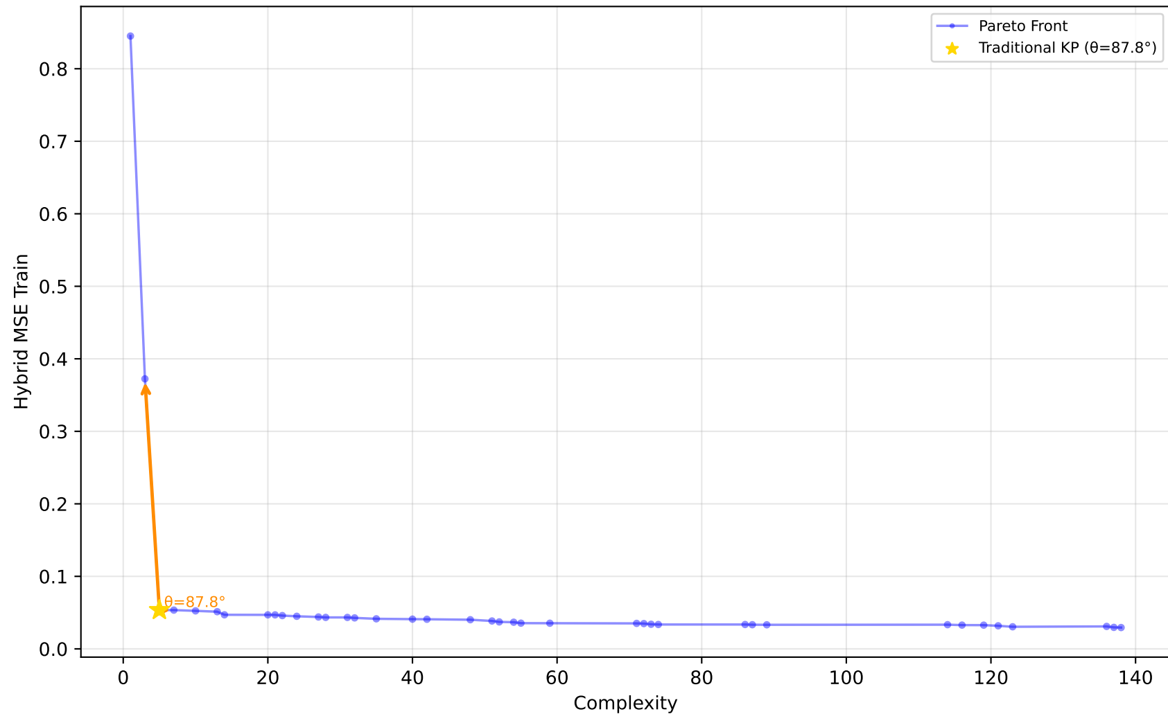
519_vinnie - Run 5 - SVP - Hybrid MSE Train \lambda_1=0.00, \lambda_2=0.00, \lambda_3=0.00 | Difficulty: 0.50 | Method: mckp
