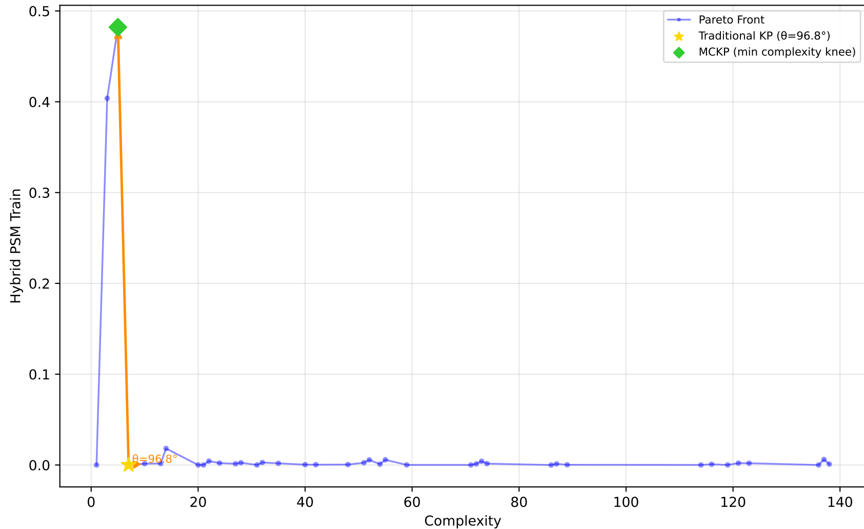
519_vinnie - Run 5 - SVP - Hybrid PSM Train \lambda_1=0.00, \lambda_2=0.00, \lambda_3=0.00 | Difficulty: 0.50 | Method: mckp
