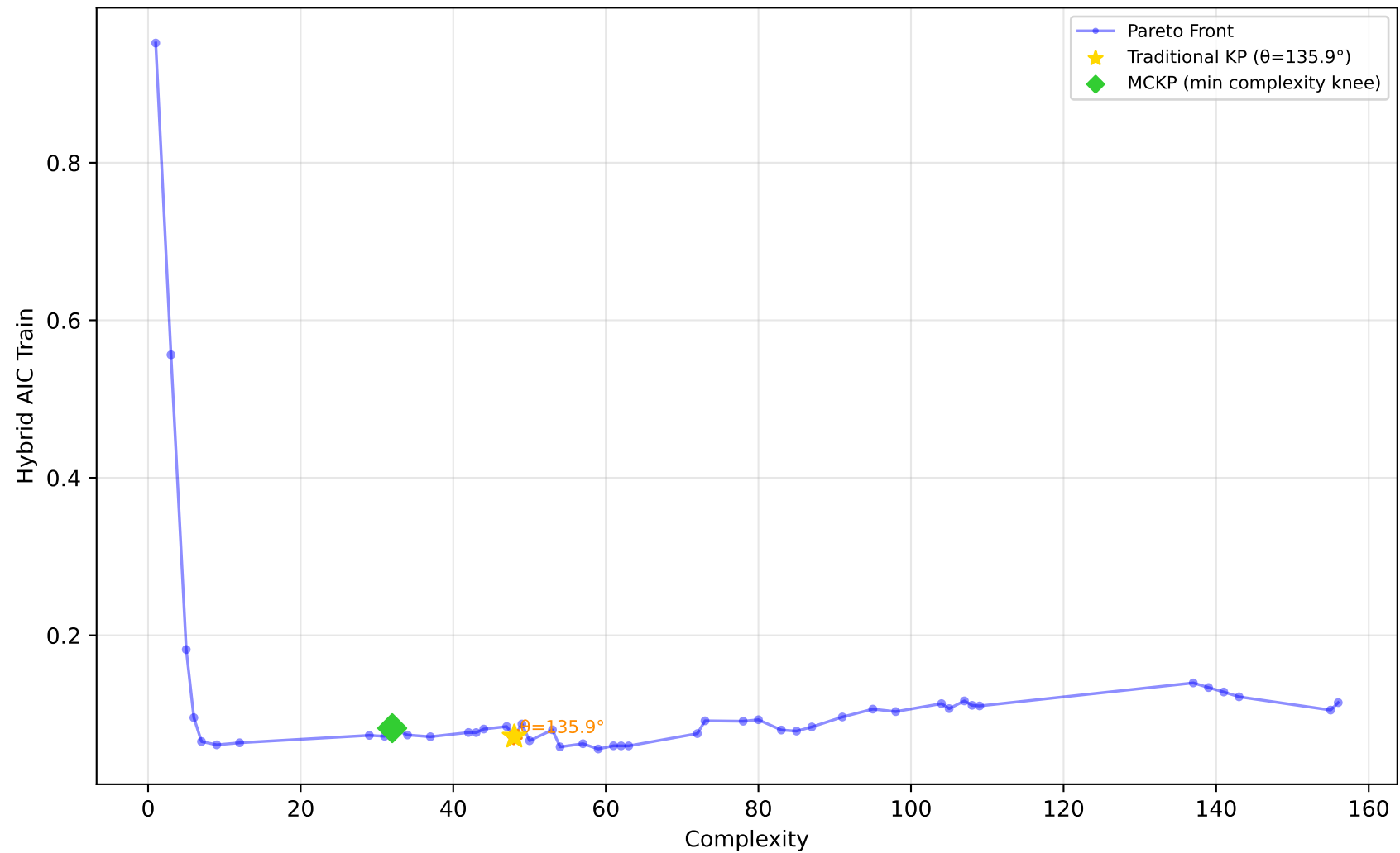
519_vinnie - Run 6 - MVP - Hybrid AIC Train \lambda_1=0.00, \lambda_2=0.10, \lambda_3=0.00 | Difficulty: 0.73 | Method: hmr
