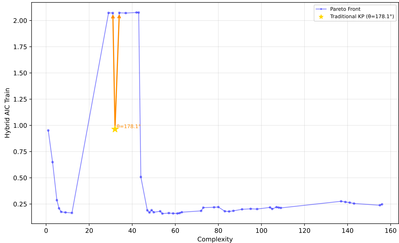
519_vinnie - Run 6 - MVP - Hybrid AIC Train \lambda_1=1.00, \lambda_2=0.00, \lambda_3=1.00 | Difficulty: 0.73 | Method: hmr
