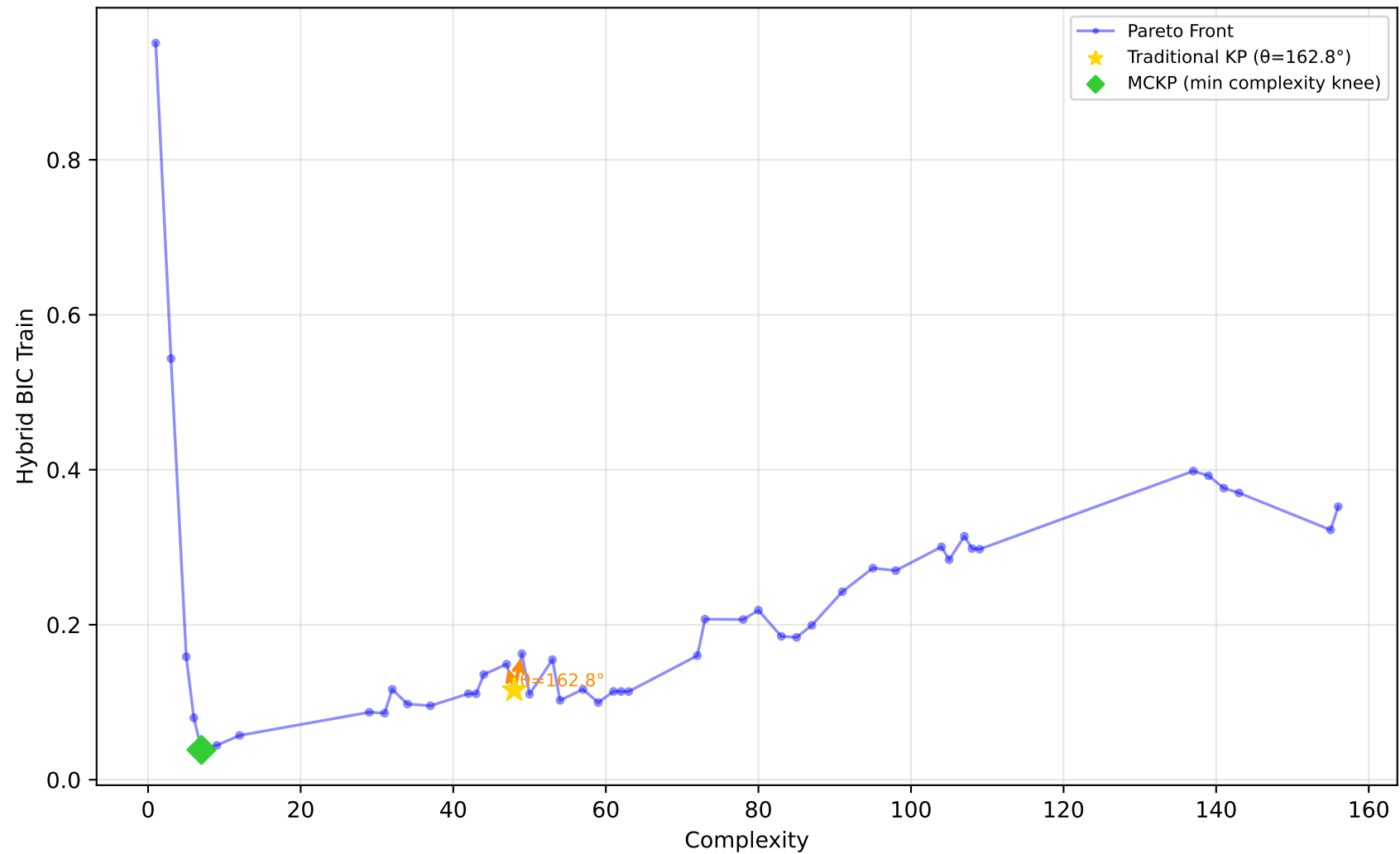
519_vinnie - Run 6 - MVP - Hybrid BIC Train \lambda_1=0.00, \lambda_2=0.10, \lambda_3=0.00 | Difficulty: 0.73 | Method: hmr
