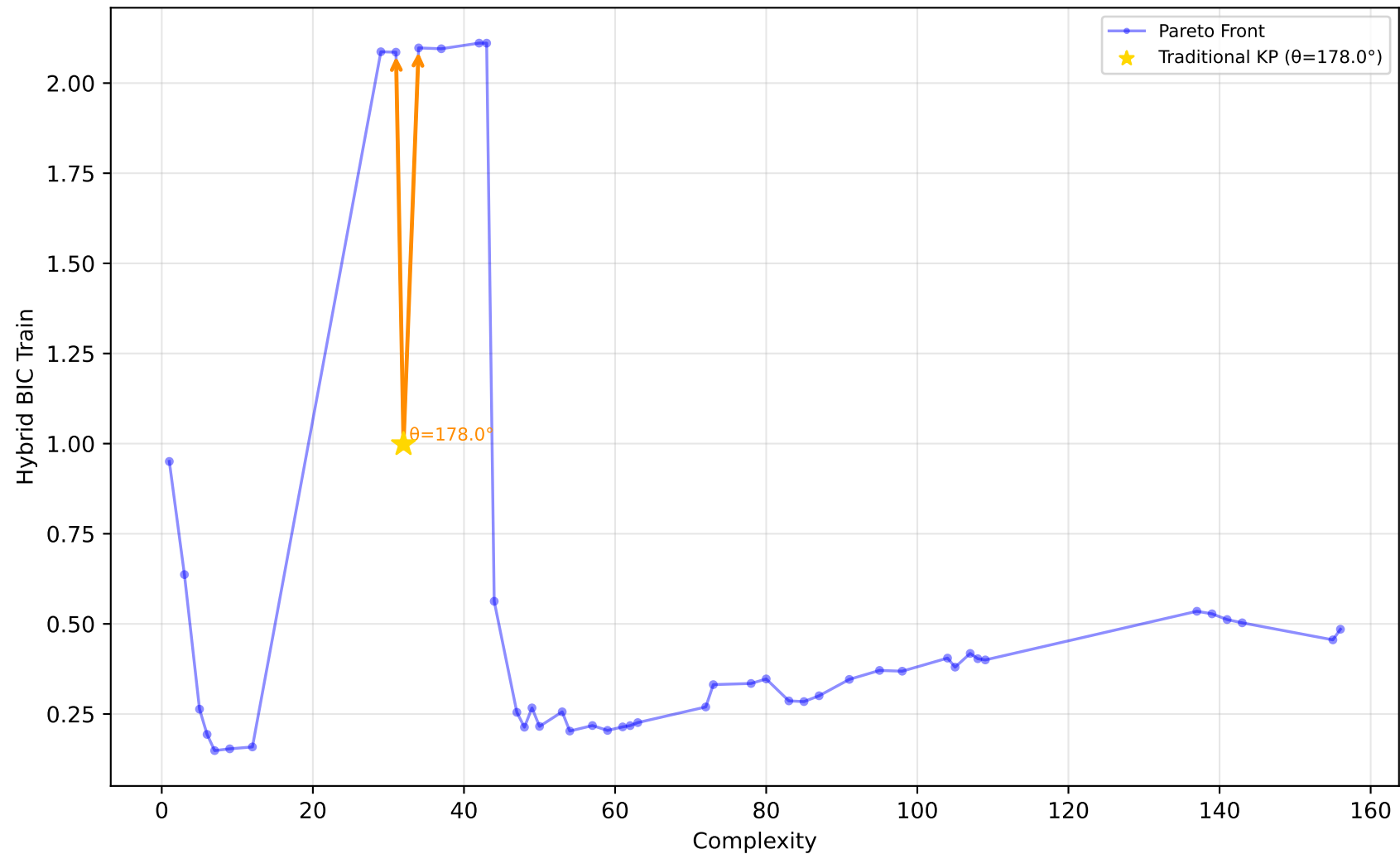
519_vinnie - Run 6 - MVP - Hybrid BIC Train \lambda_1=1.00, \lambda_2=0.00, \lambda_3=1.00 | Difficulty: 0.73 | Method: hmr
