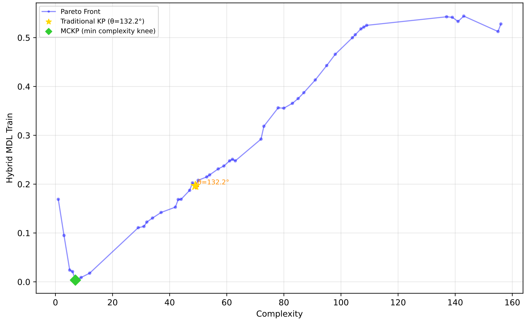
519_vinnie - Run 6 - MVP - Hybrid MDL Train \lambda_1=0.00, \lambda_2=0.10, \lambda_3=0.00 | Difficulty: 0.73 | Method: hmr
