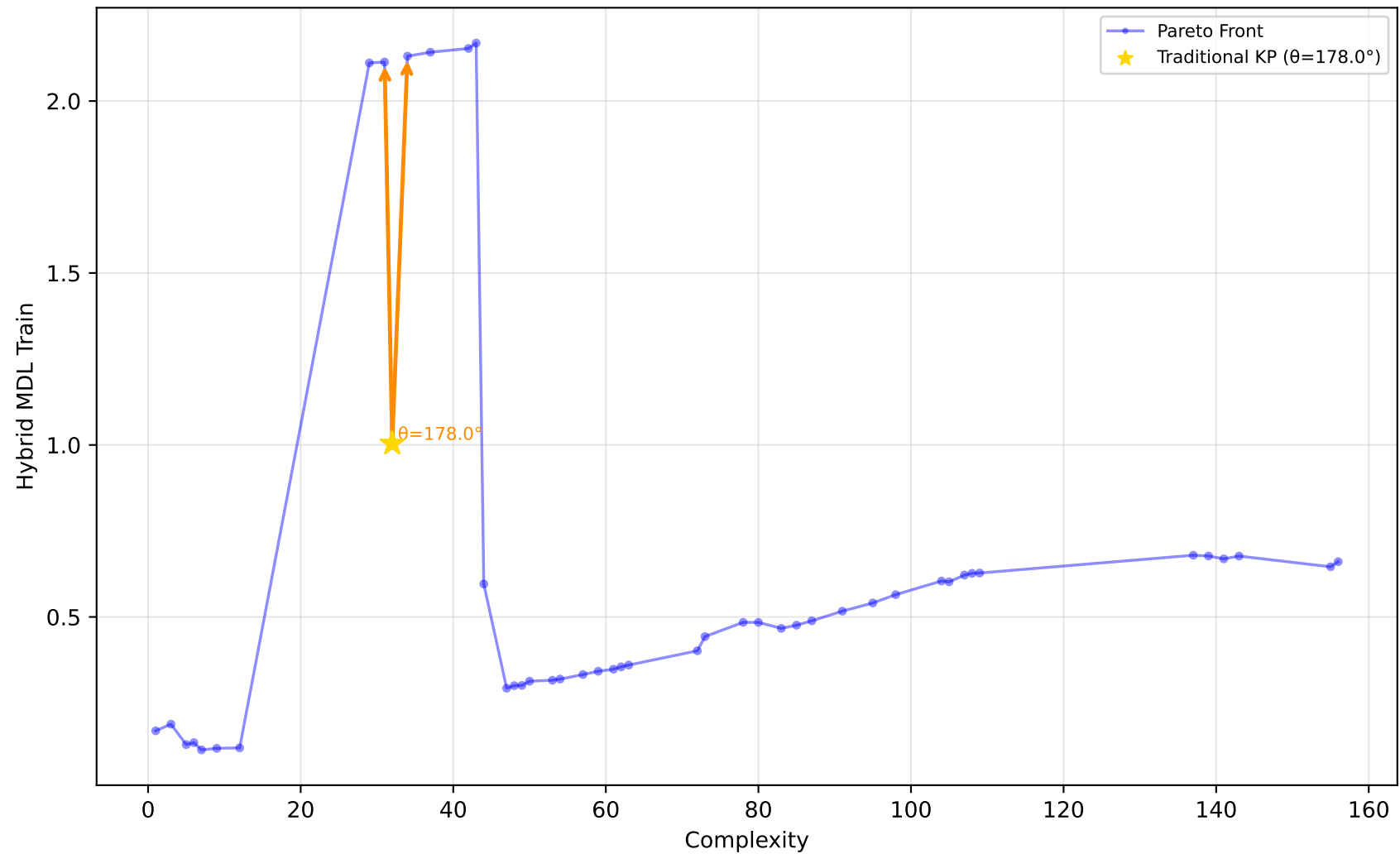
519_vinnie - Run 6 - MVP - Hybrid MDL Train \lambda_1=1.00, \lambda_2=0.00, \lambda_3=1.00 | Difficulty: 0.73 | Method: hmr
