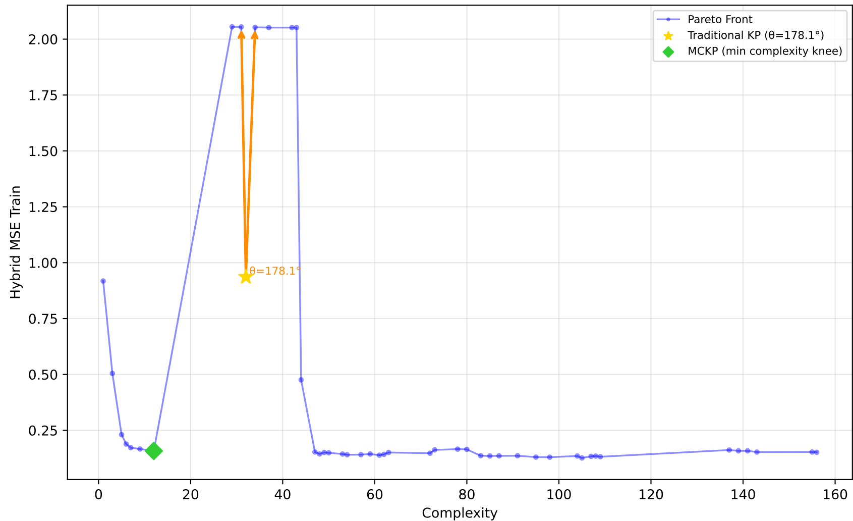
519_vinnie - Run 6 - MVP - Hybrid MSE Train \lambda_1=1.00 , \lambda_2=0.00 , \lambda_3=1.00 | Difficulty: 0.73 | Method: hmr
