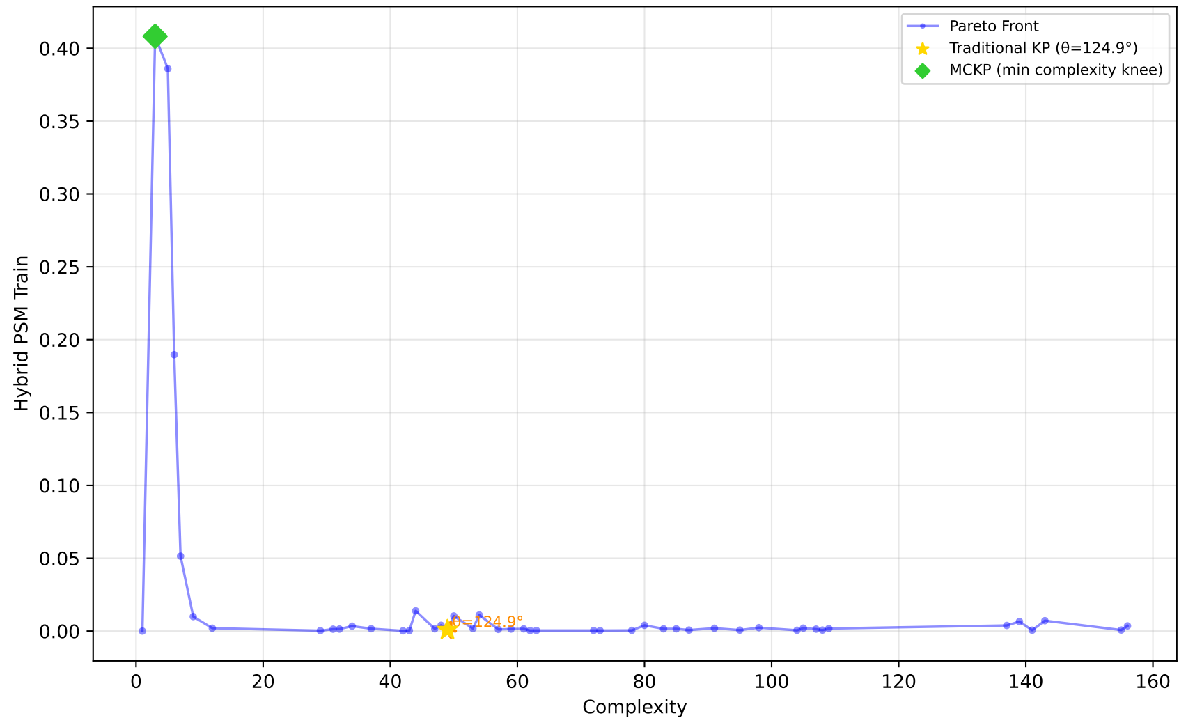
519_vinnie - Run 6 - MVP - Hybrid PSM Train \lambda_1=0.00, \lambda_2=0.10, \lambda_3=0.00 | Difficulty: 0.73 | Method: hmr
