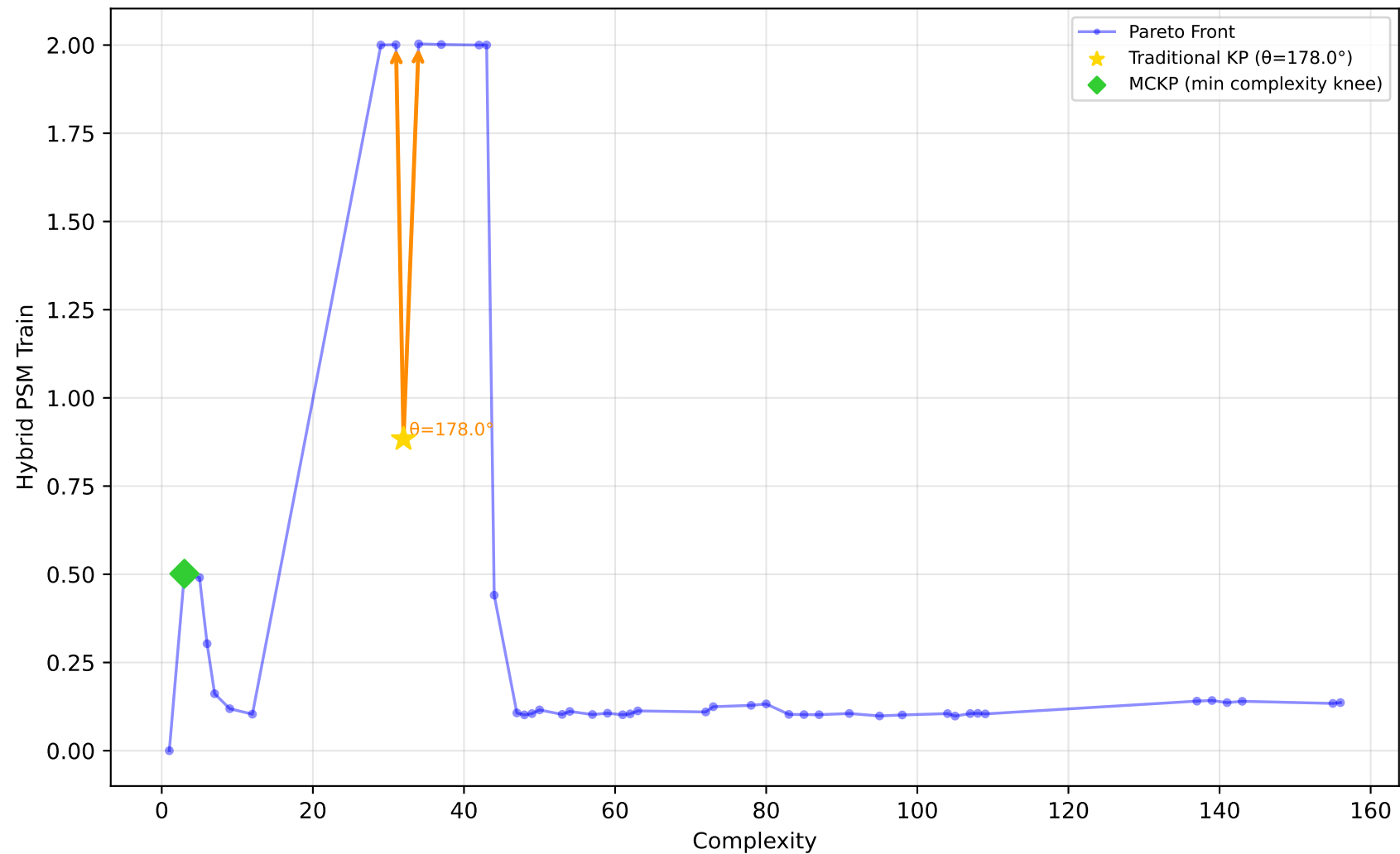
519_vinnie - Run 6 - MVP - Hybrid PSM Train \lambda_1=1.00, \lambda_2=0.00, \lambda_3=1.00 | Difficulty: 0.73 | Method: hmr
