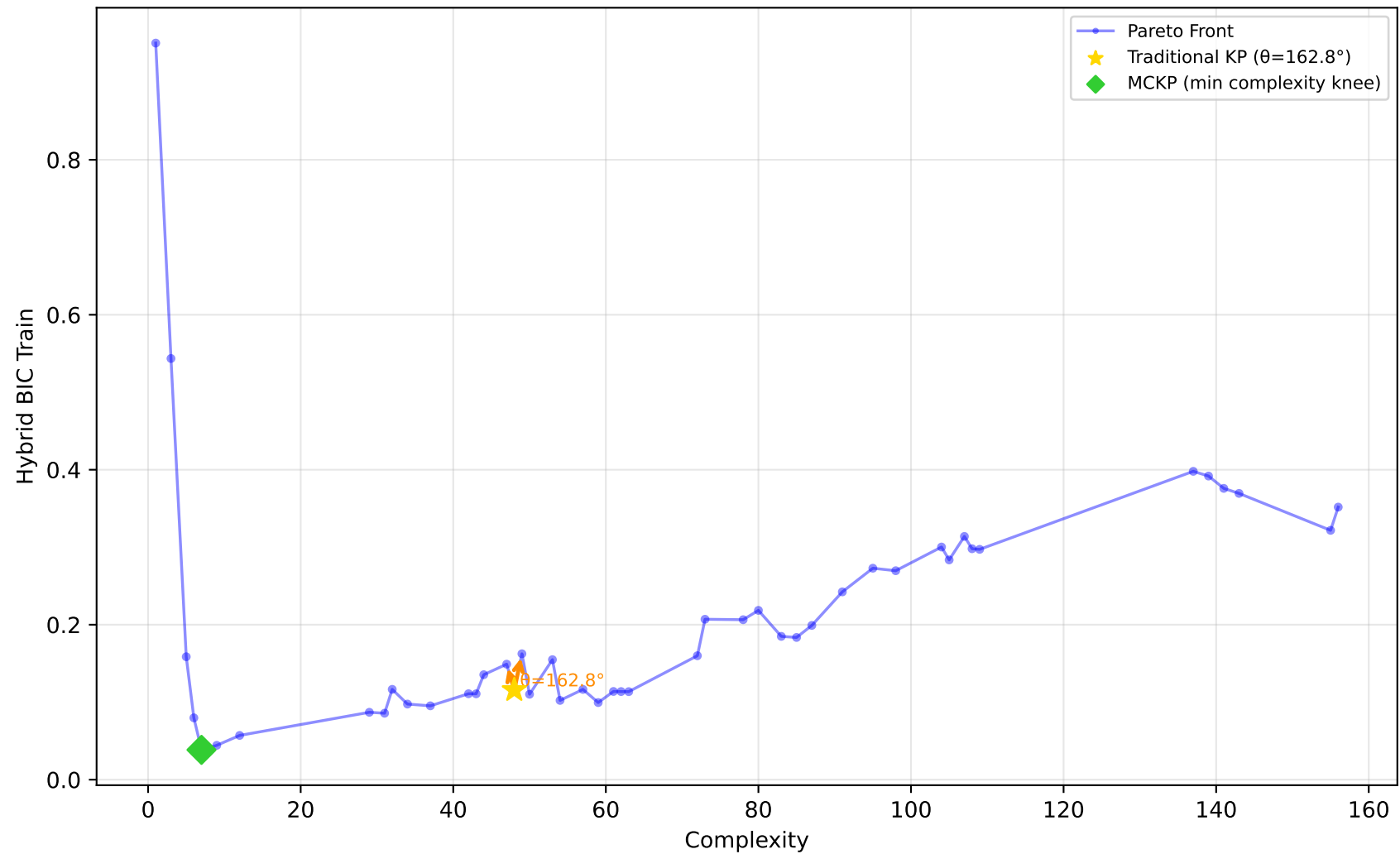
519_vinnie - Run 6 - SVP - Hybrid BIC Train \lambda_1=0.00, \lambda_2=0.00, \lambda_3=0.00 | Difficulty: 0.73 | Method: hmr
