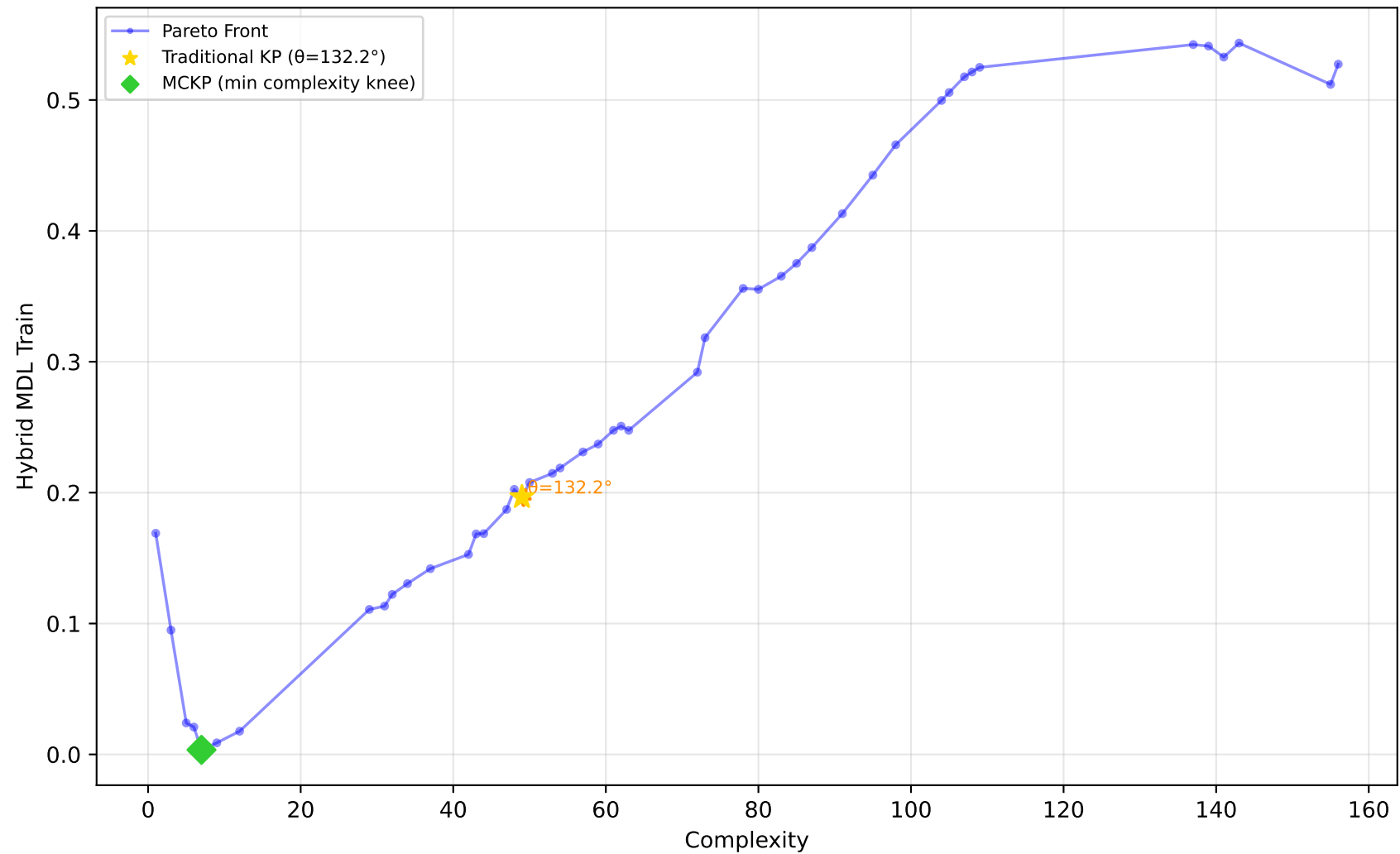
519_vinnie - Run 6 - SVP - Hybrid MDL Train \lambda_1=0.00, \lambda_2=0.00, \lambda_3=0.00 | Difficulty: 0.73 | Method: hmr
