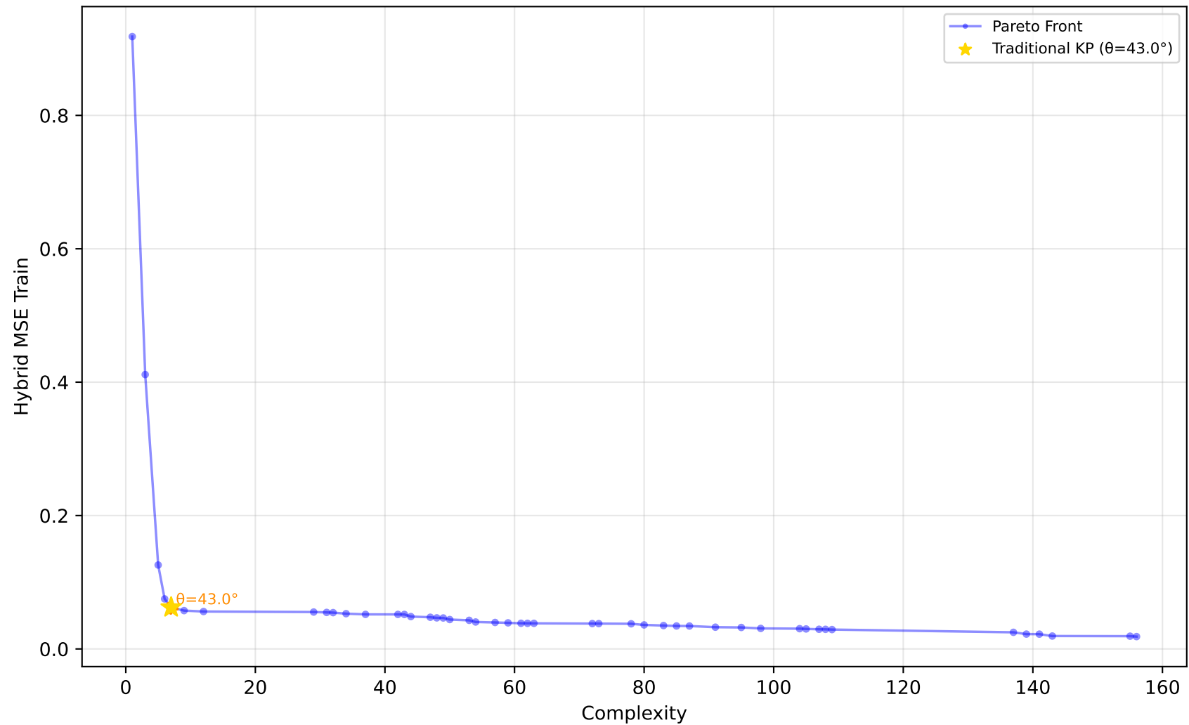
519_vinnie - Run 6 - SVP - Hybrid MSE Train \lambda_1=0.00, \lambda_2=0.00, \lambda_3=0.00 | Difficulty: 0.73 | Method: hmr
