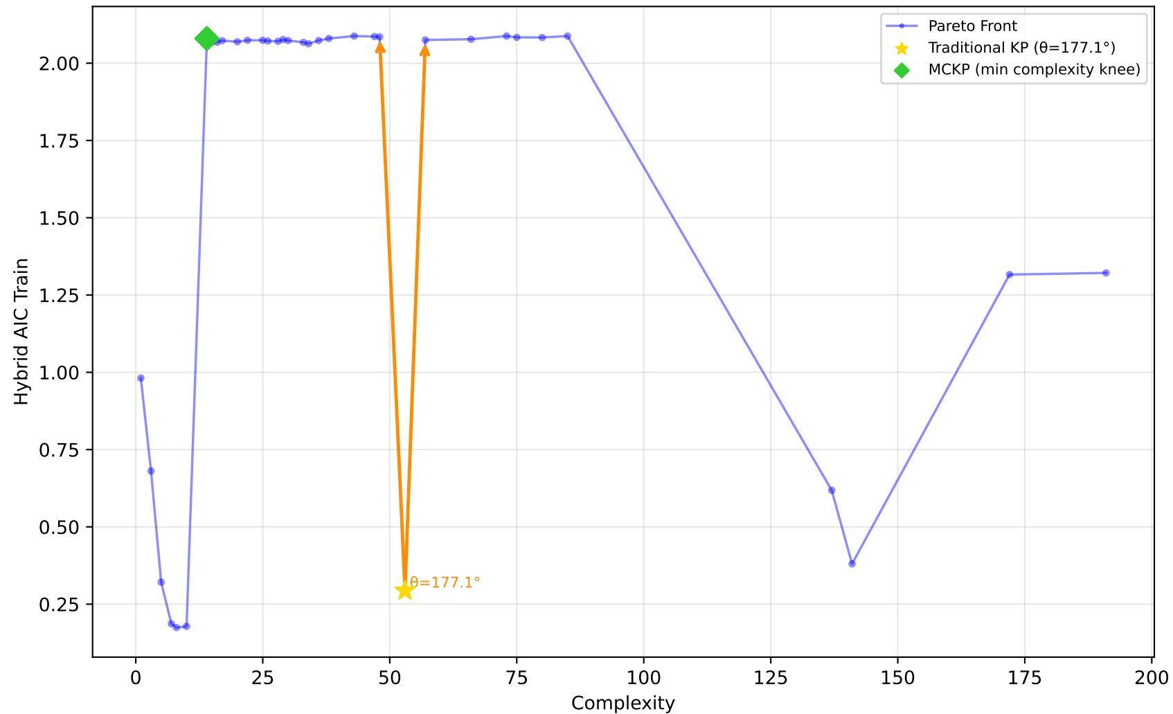
519_vinnie - Run 7 - MVP - Hybrid AIC Train \lambda_1=1.00, \lambda_2=0.00, \lambda_3=1.00 | Difficulty: 0.70 | Method: hmr
