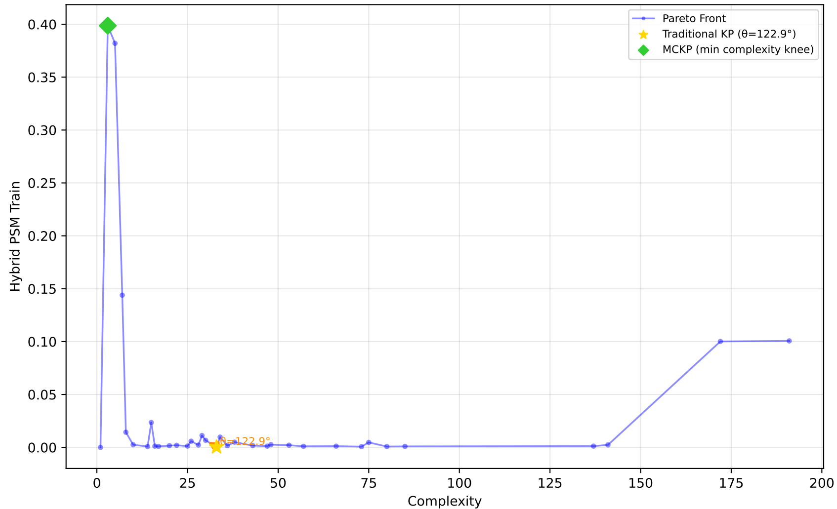
519_vinnie - Run 7 - MVP - Hybrid PSM Train \lambda_1=0.00, \lambda_2=0.10, \lambda_3=0.00 | Difficulty: 0.70 | Method: hmr
