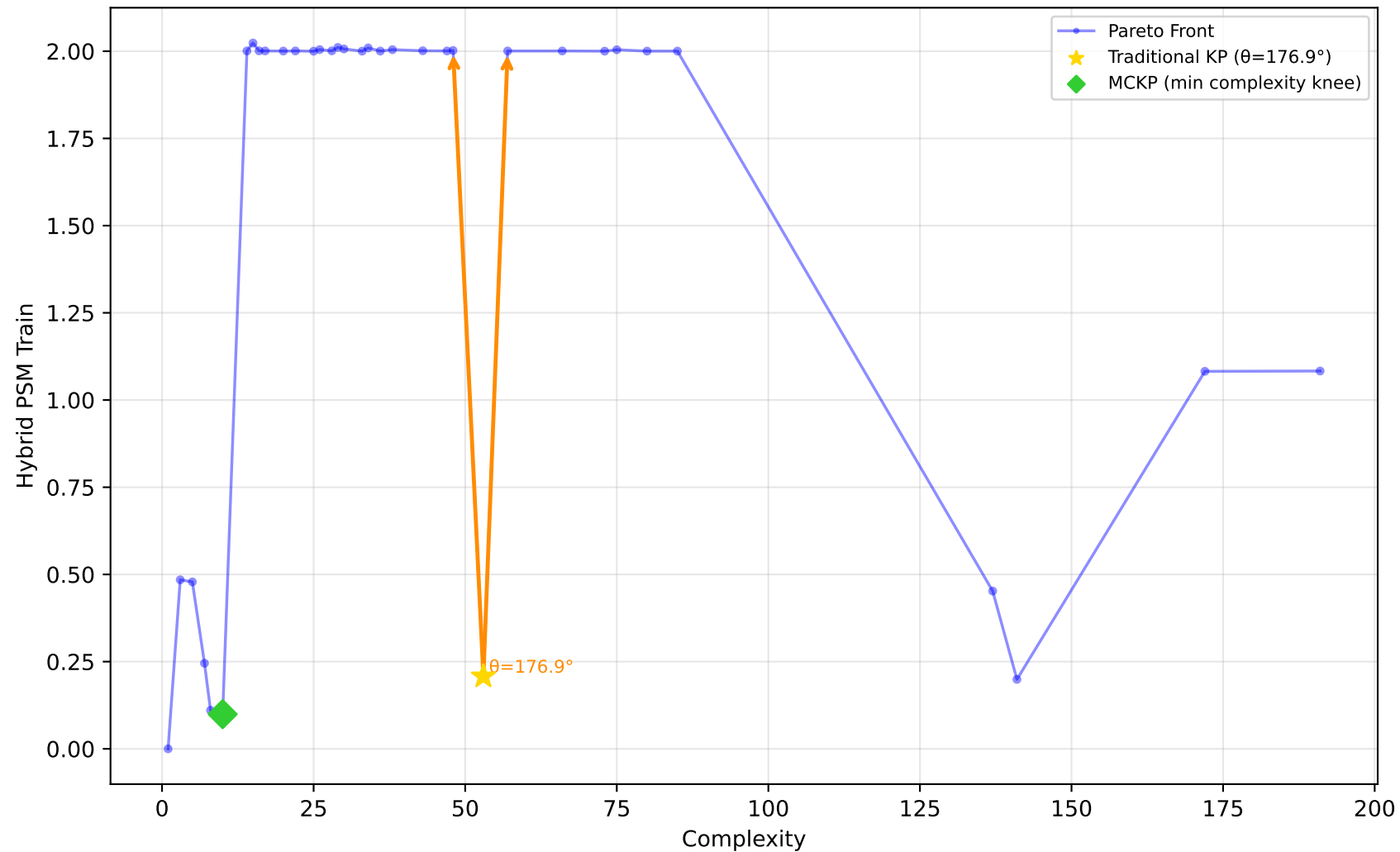
519_vinnie - Run 7 - MVP - Hybrid PSM Train \lambda_1=1.00, \lambda_2=0.00, \lambda_3=1.00 | Difficulty: 0.70 | Method: hmr
