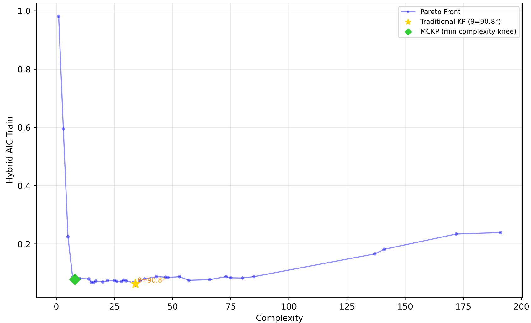
519_vinnie - Run 7 - SVP - Hybrid AIC Train \lambda_1=0.00, \lambda_2=0.00, \lambda_3=0.00 | Difficulty: 0.70 | Method: hmr
