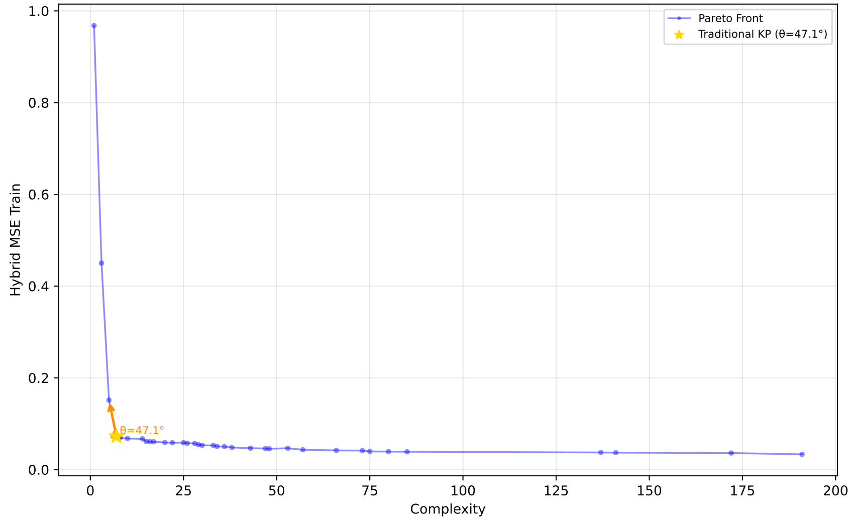
519_vinnie - Run 7 - SVP - Hybrid MSE Train \lambda_1=0.00, \lambda_2=0.00, \lambda_3=0.00 | Difficulty: 0.70 | Method: hmr
