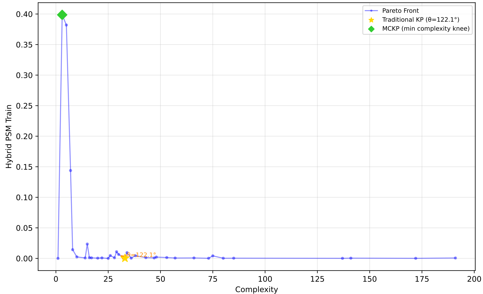
519_vinnie - Run 7 - SVP - Hybrid PSM Train \lambda_1=0.00, \lambda_2=0.00, \lambda_3=0.00 | Difficulty: 0.70 | Method: hmr
