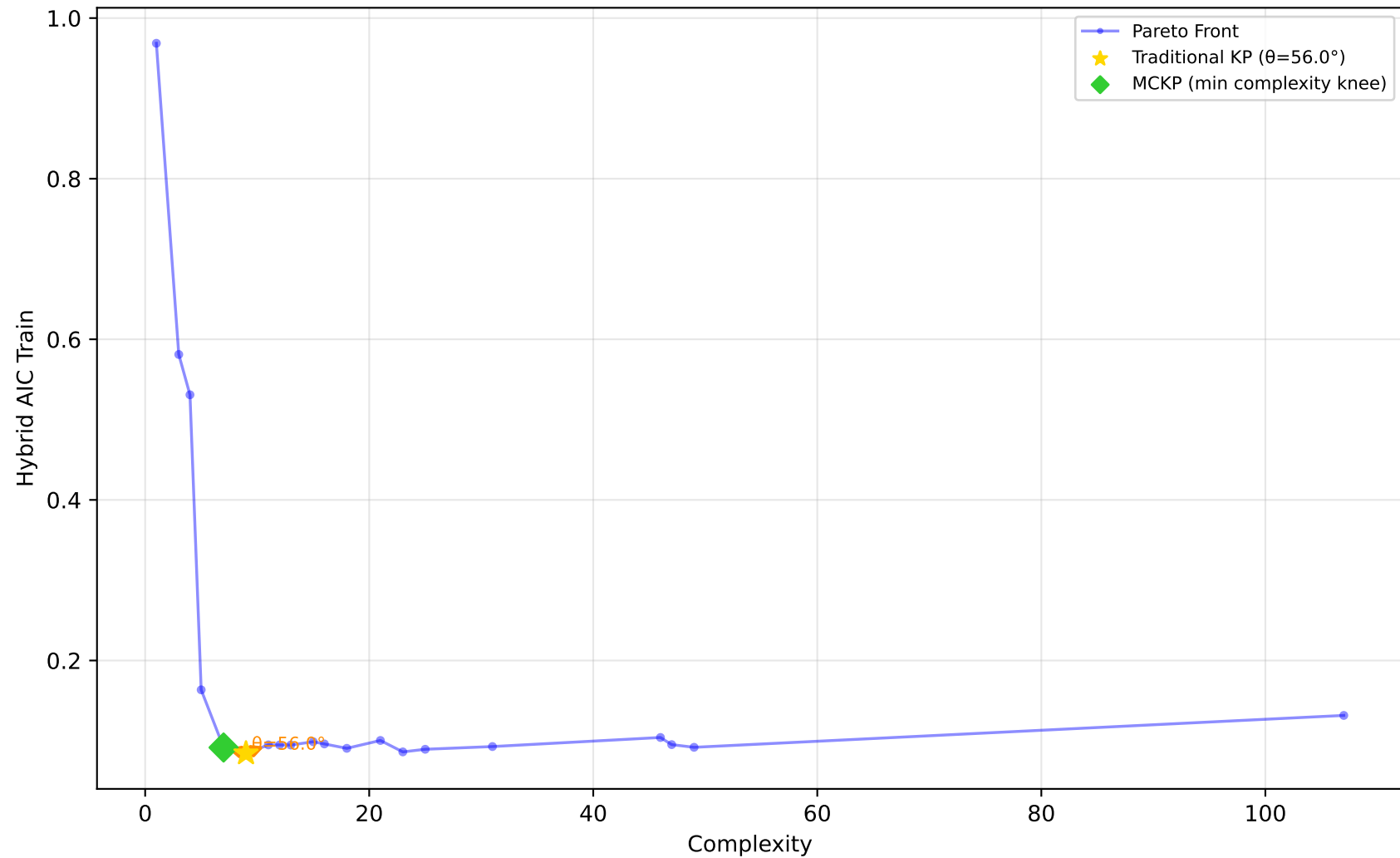
519_vinnie - Run 8 - MVP - Hybrid AIC Train \lambda_1=0.00, \lambda_2=0.10, \lambda_3=0.00 | Difficulty: 1.00 | Method: hmr
