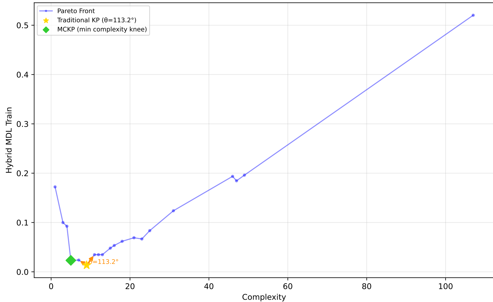
519_vinnie - Run 8 - MVP - Hybrid MDL Train \lambda_1=0.00, \lambda_2=0.10, \lambda_3=0.00 | Difficulty: 1.00 | Method: hmr
