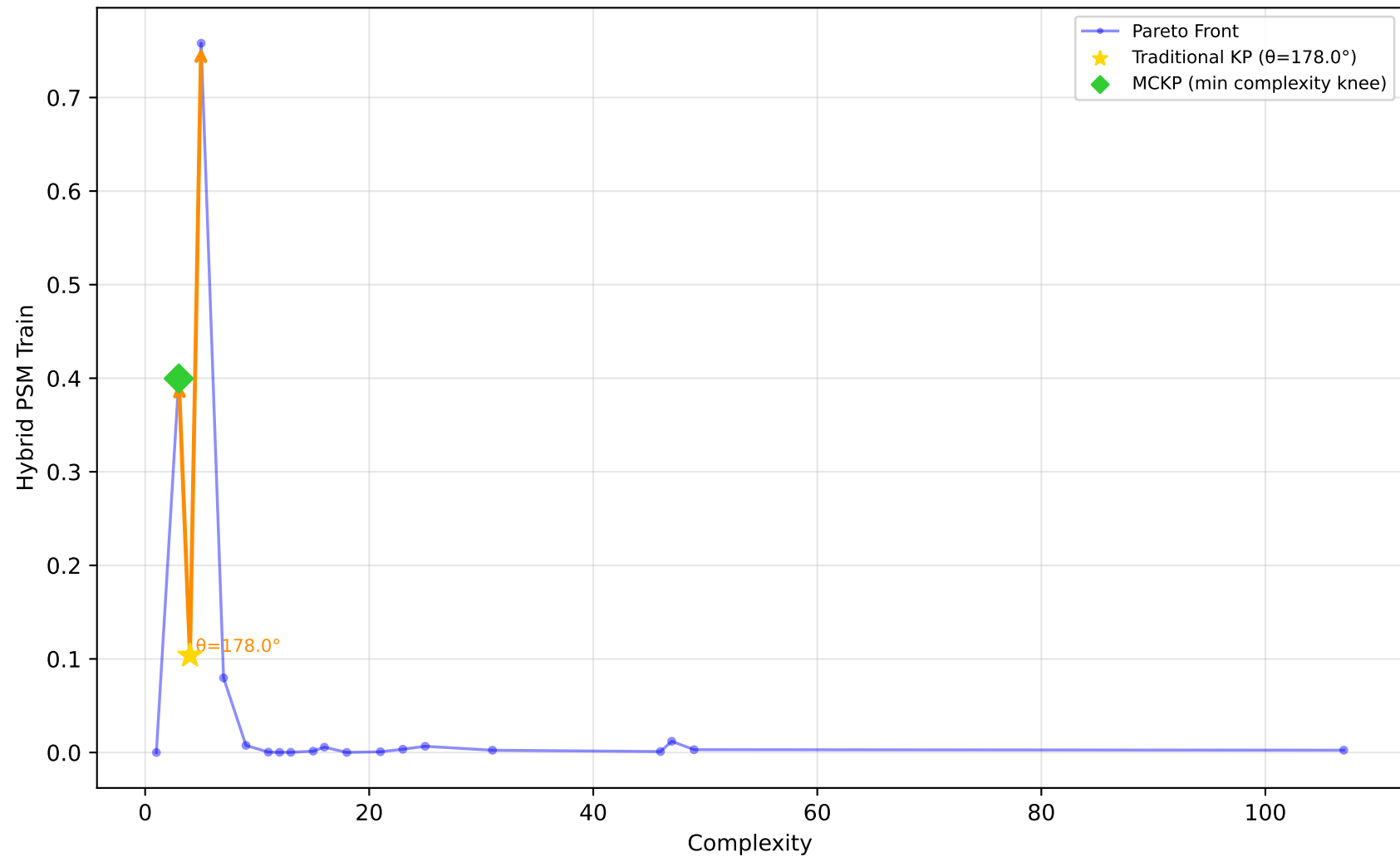
519_vinnie - Run 8 - MVP - Hybrid PSM Train \lambda_1=0.00, \lambda_2=0.10, \lambda_3=0.00 | Difficulty: 1.00 | Method: hmr
