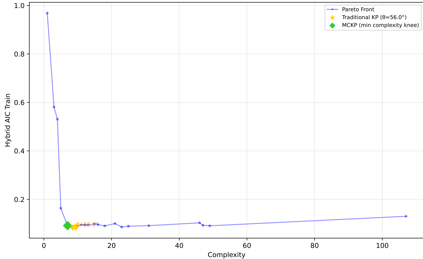
519_vinnie - Run 8 - SVP - Hybrid AIC Train \lambda_1=0.00, \lambda_2=0.00, \lambda_3=0.00 | Difficulty: 1.00 | Method: hmr
