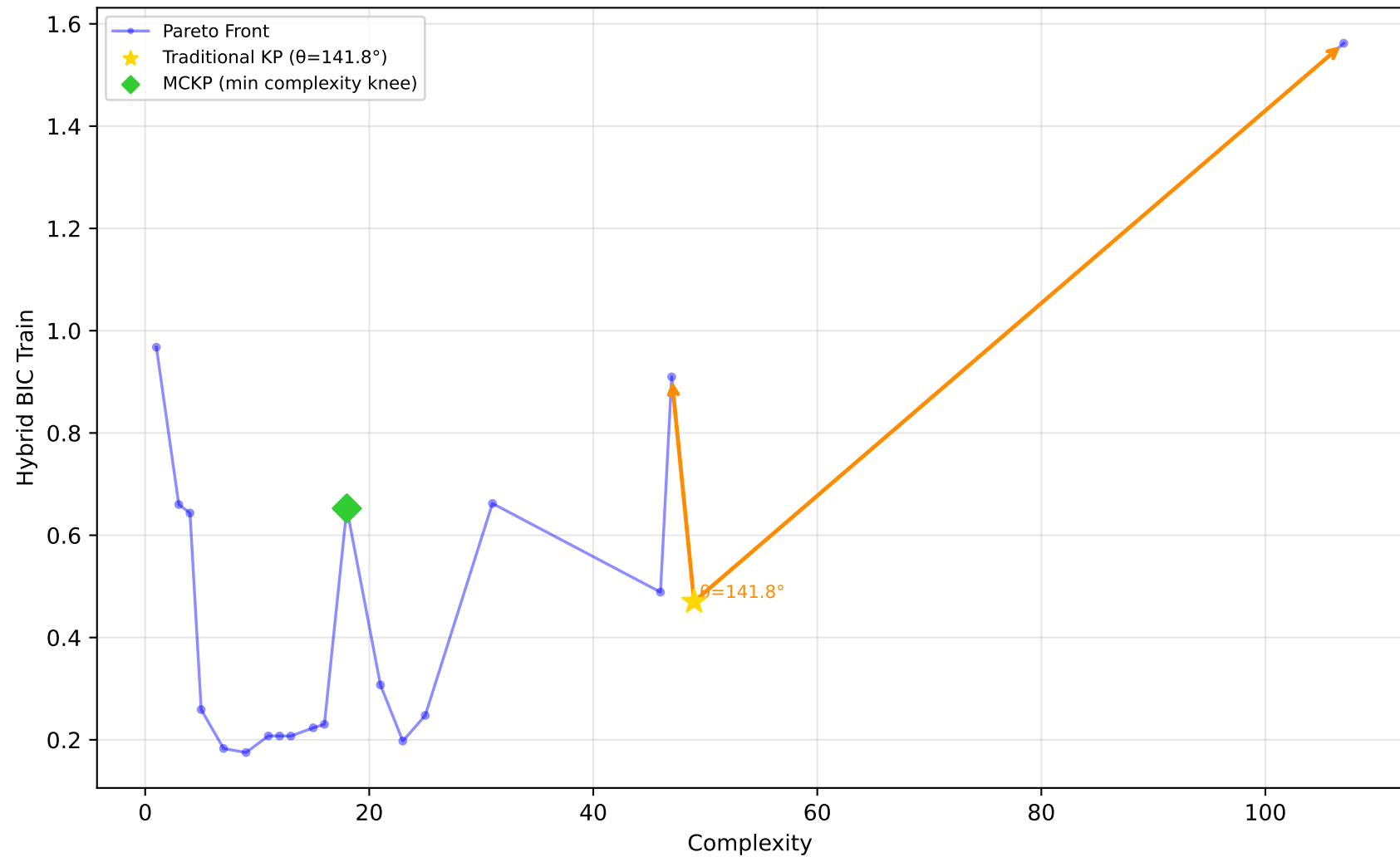
519_vinnie - Run 8 - SVP - Hybrid BIC Train \lambda_1=1.00, \lambda_2=1.00, \lambda_3=1.00 | Difficulty: 1.00 | Method: hmr
