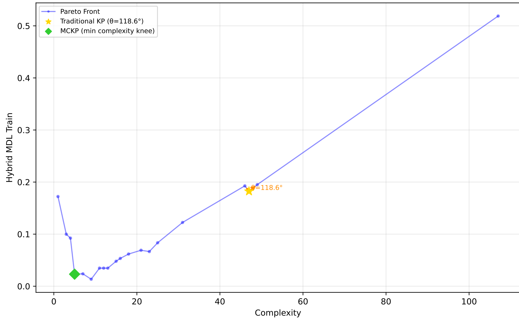
519_vinnie - Run 8 - SVP - Hybrid MDL Train \lambda_1=0.00, \lambda_2=0.00, \lambda_3=0.00 | Difficulty: 1.00 | Method: hmr
