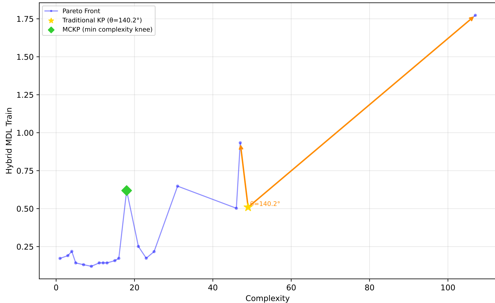
519_vinnie - Run 8 - SVP - Hybrid MDL Train \lambda_1=1.00, \lambda_2=1.00, \lambda_3=1.00 | Difficulty: 1.00 | Method: hmr
