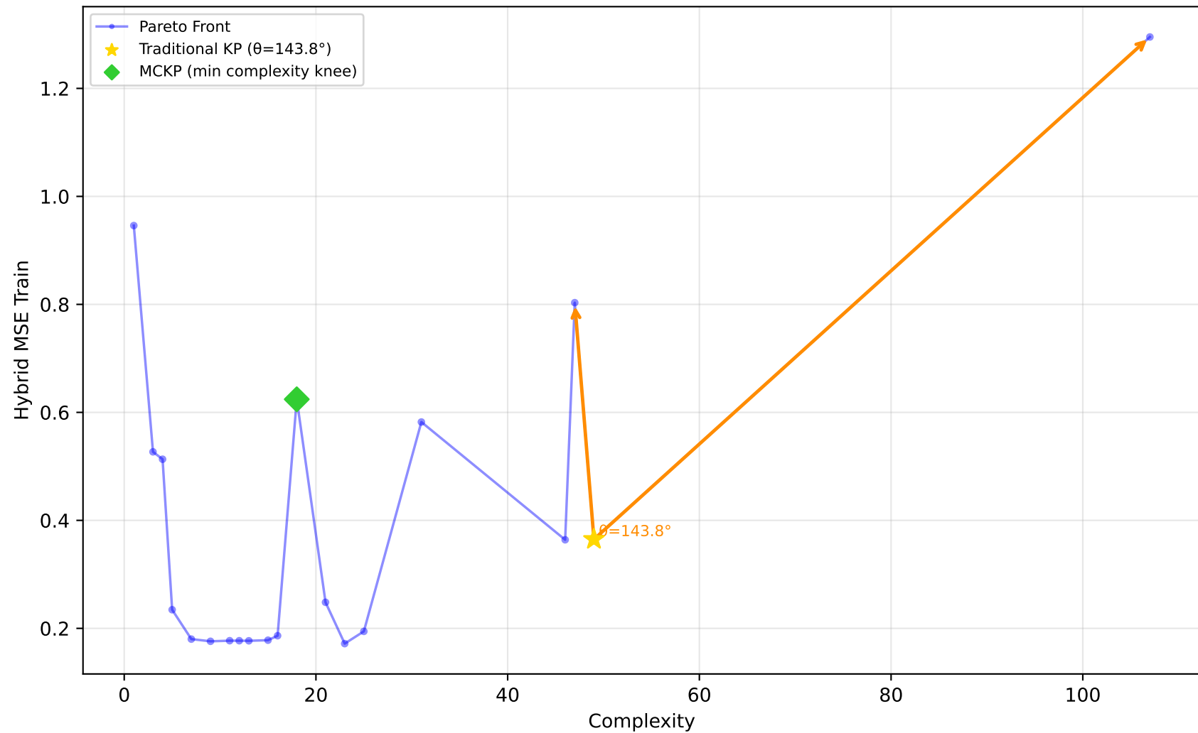
519_vinnie - Run 8 - SVP - Hybrid MSE Train \lambda_1=1.00, \lambda_2=1.00, \lambda_3=1.00 | Difficulty: 1.00 | Method: hmr
