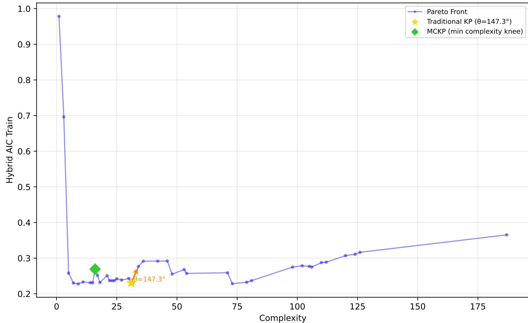
519_vinnie - Run 9 - MVP - Hybrid AIC Train \lambda_1=1.00, \lambda_2=0.00, \lambda_3=1.00 | Difficulty: 0.60 | Method: hmr
