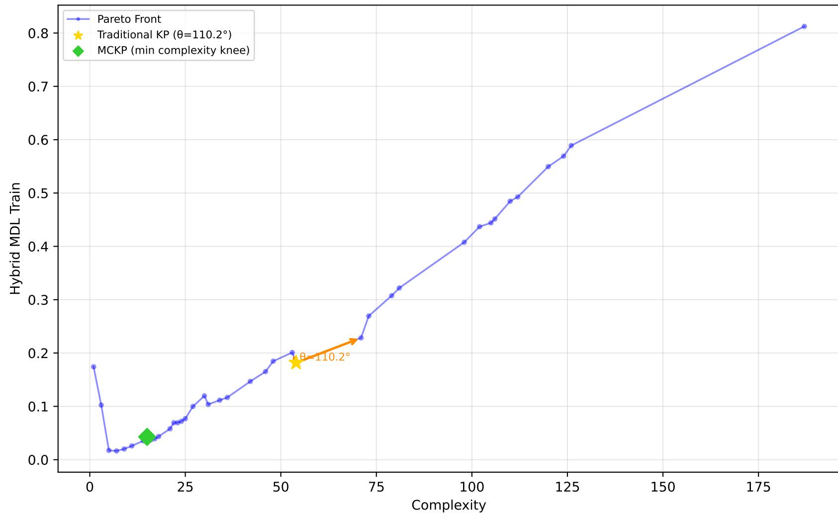
519_vinnie - Run 9 - MVP - Hybrid MDL Train \lambda_1=0.00, \lambda_2=0.10, \lambda_3=0.00 | Difficulty: 0.60 | Method: hmr
