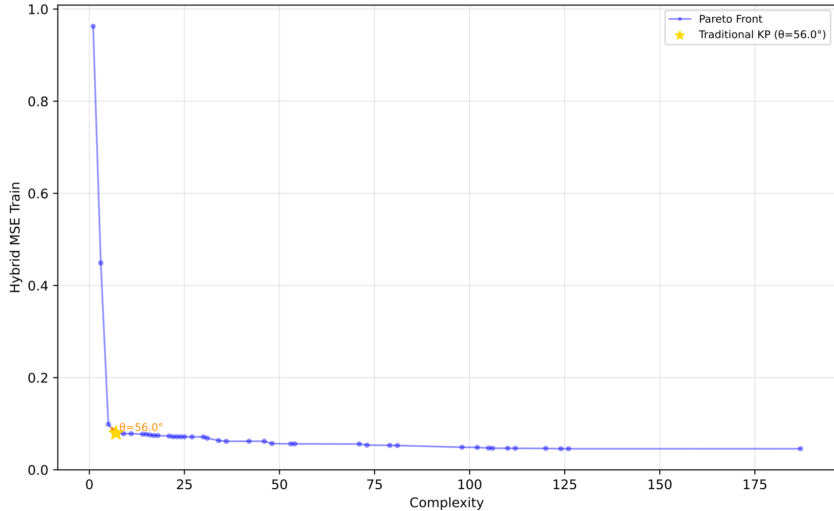
519_vinnie - Run 9 - MVP - Hybrid MSE Train \lambda_1=0.00, \lambda_2=0.10, \lambda_3=0.00 | Difficulty: 0.60 | Method: hmr
