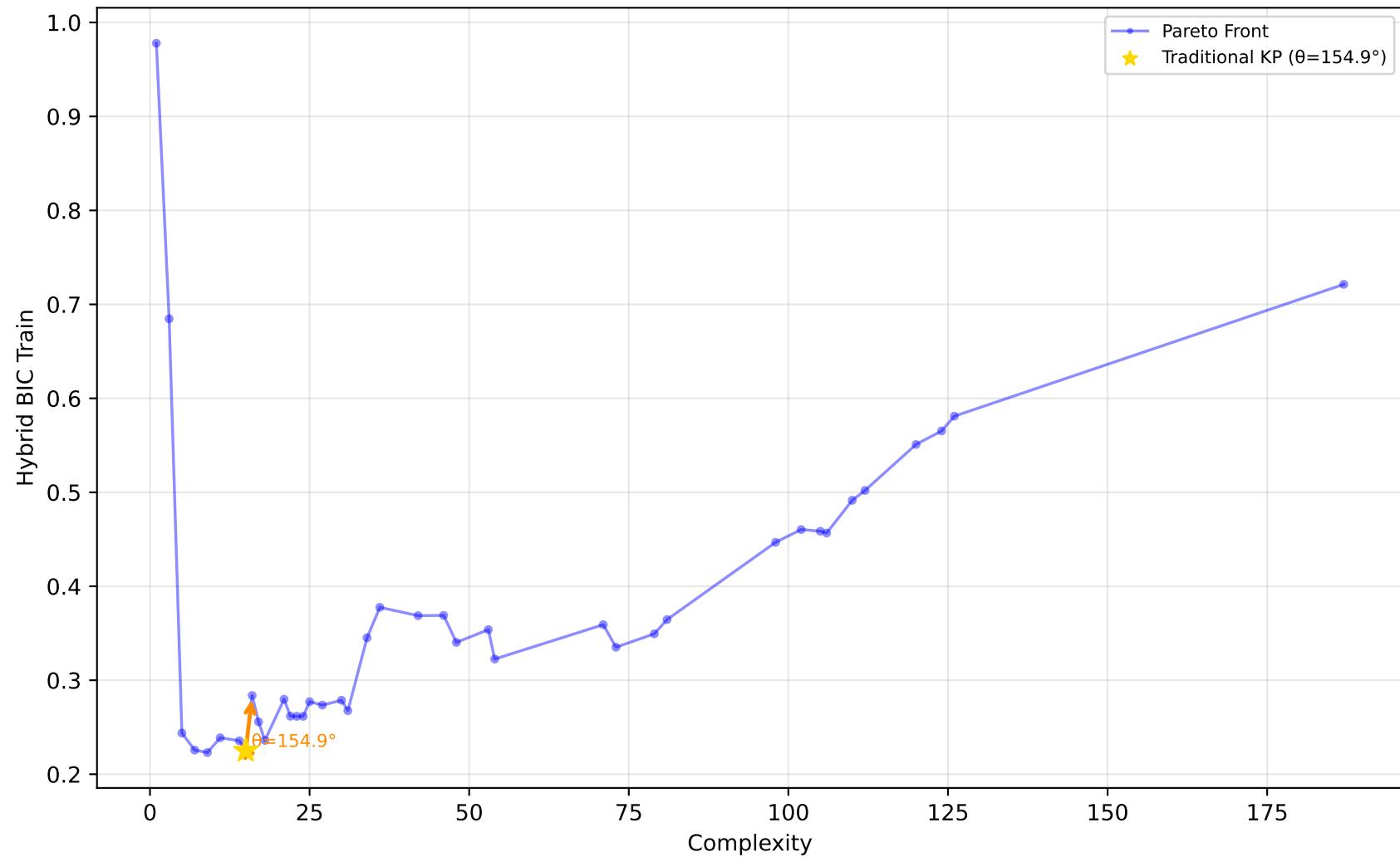
519_vinnie - Run 9 - SVP - Hybrid BIC Train \lambda_1=1.00, \lambda_2=1.00, \lambda_3=1.00 | Difficulty: 0.60 | Method: hmr
