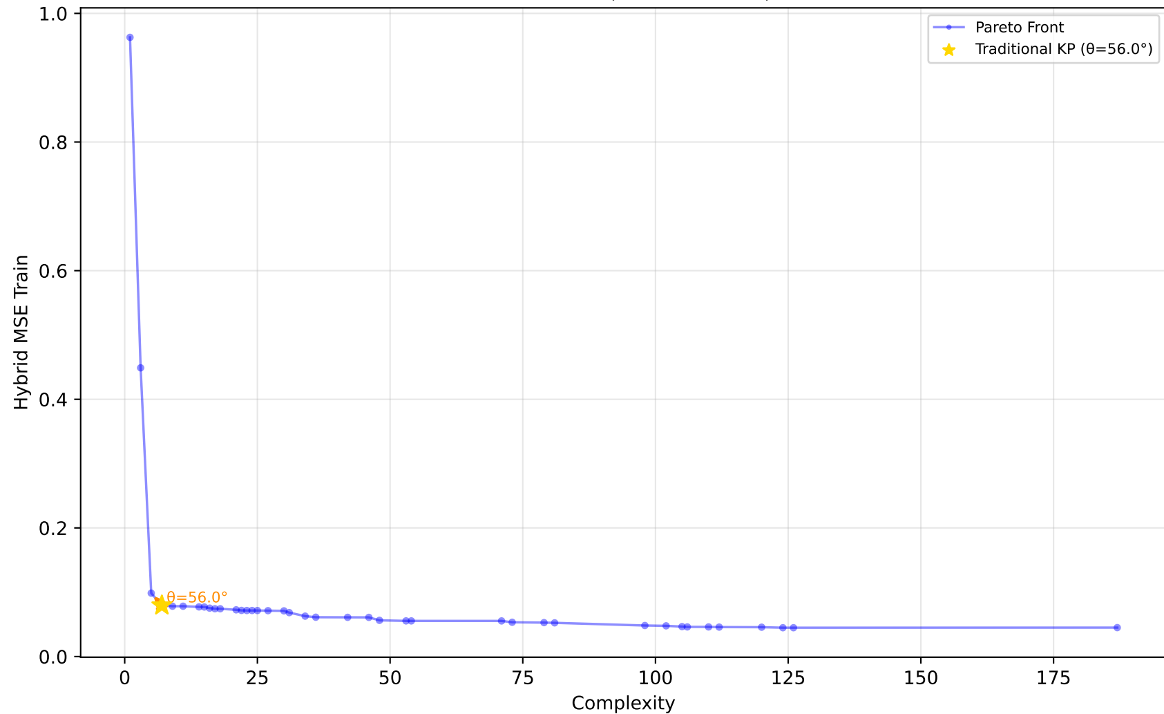
519_vinnie - Run 9 - SVP - Hybrid MSE Train \lambda_1=0.00, \lambda_2=0.00, \lambda_3=0.00 | Difficulty: 0.60 | Method: hmr
