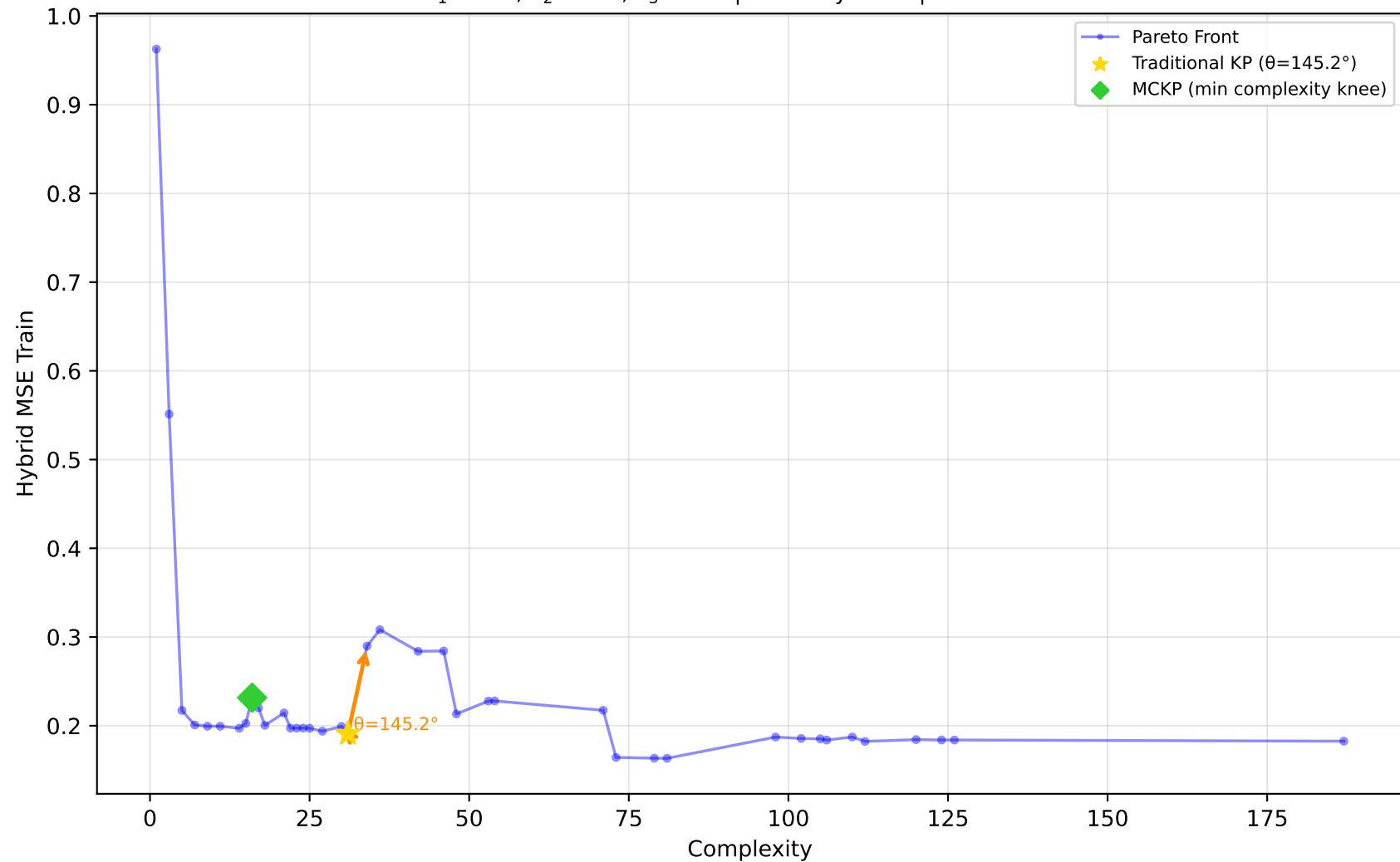
519_vinnie - Run 9 - SVP - Hybrid MSE Train \lambda_1=1.00, \lambda_2=1.00, \lambda_3=1.00 | Difficulty: 0.60 | Method: hmr
