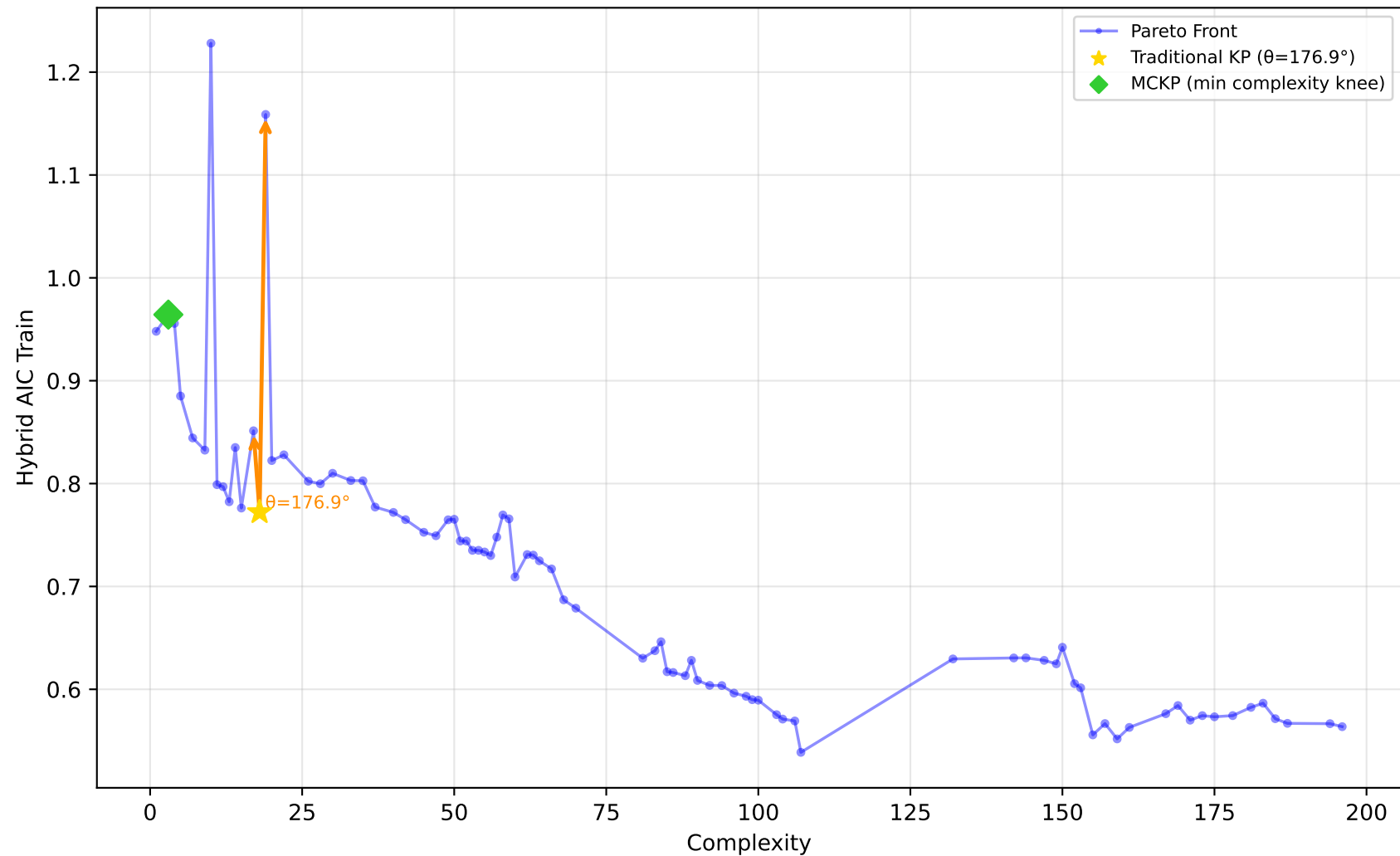
542_pollution - Run 10 - MVP - Hybrid AIC Train \lambda_1=0.40, \lambda_2=0.10, \lambda_3=0.00 | Difficulty: 1.00 | Method: hmr
