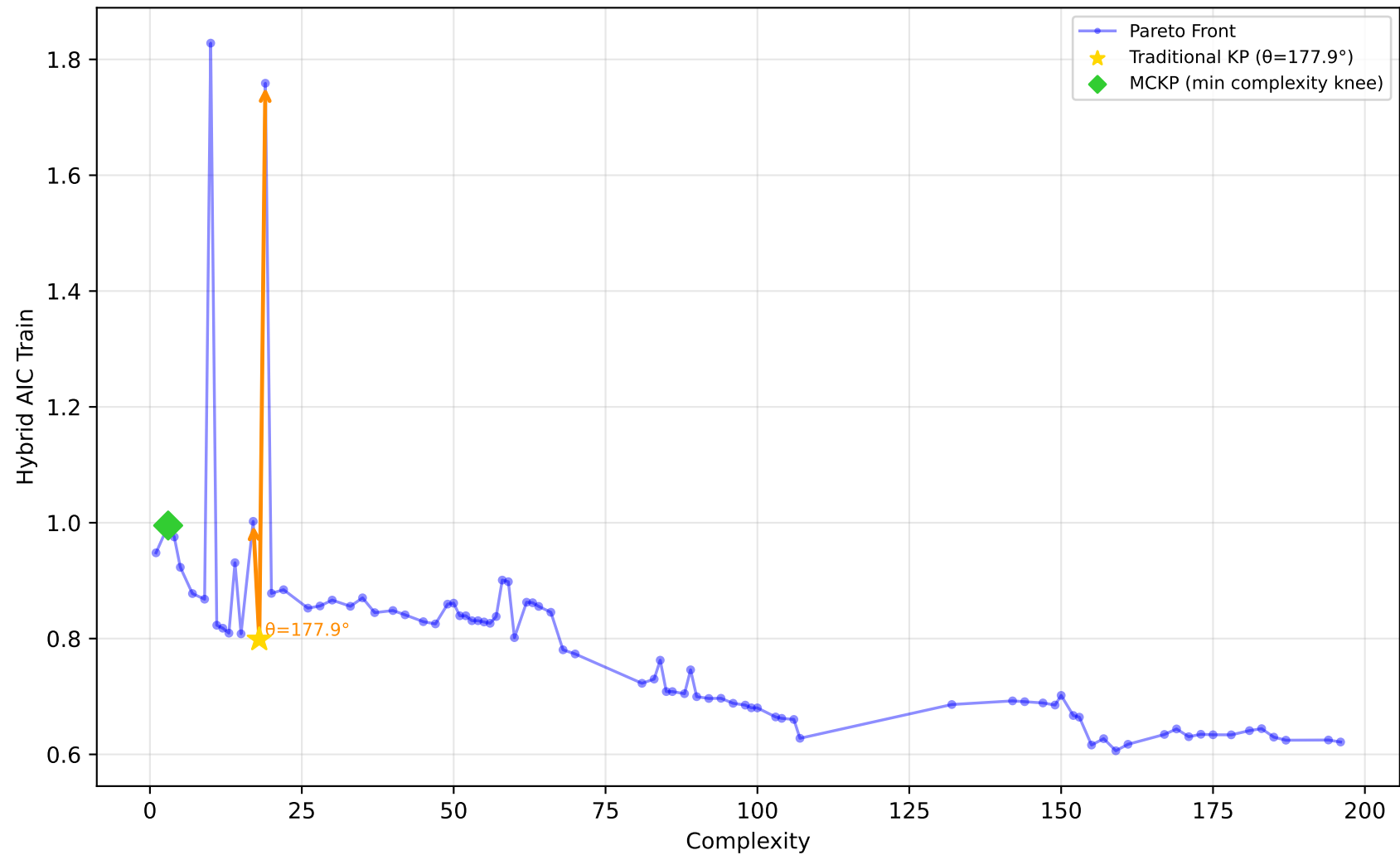
542_pollution - Run 10 - MVP - Hybrid AIC Train \lambda_1=1.00, \lambda_2=0.10, \lambda_3=0.00 | Difficulty: 1.00 | Method: hmr
